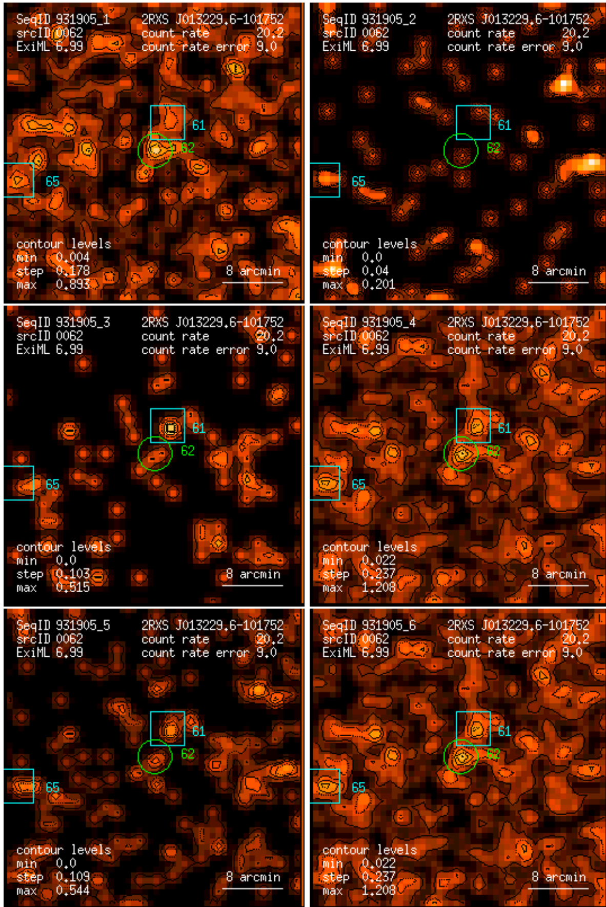
Figure 62: RASS 931905: detection 0062: band rate images, Gaussian filter: (1) PSPC channels 11 – 41, (2) 52 – 90, (3) 91 – 201, (4) 11 – 235, (5) 52 – 201, (6) 11 – 201. Broad band rates in counts/ks. Band rate contour levels in counts/ks/arcmin 2 .
