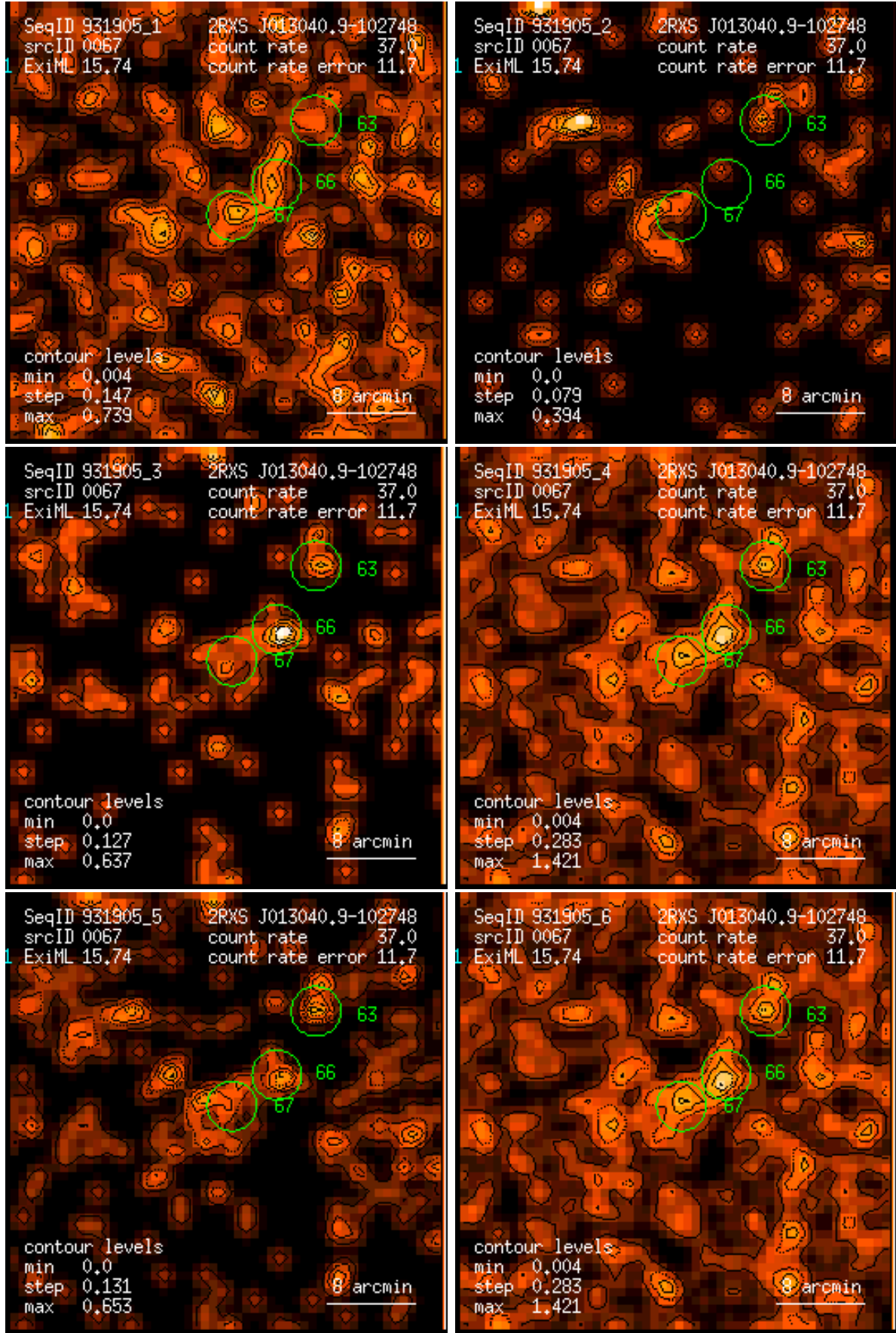
Figure 67: RASS 931905: detection 0067: band rate images, Gaussian filter: (1) PSPC channels 11 – 41, (2) 52 – 90, (3) 91 – 201, (4) 11 – 235, (5) 52 – 201, (6) 11 – 201. Broad band rates in counts/ks. Band rate contour levels in counts/ks/arcmin 2 .
