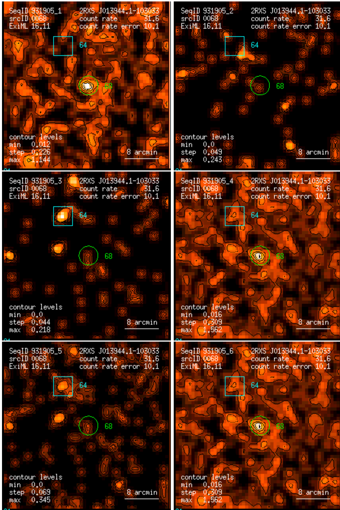
Figure 68: RASS 931905: detection 0068: band rate images, Gaussian filter: (1) PSPC channels 11 – 41, (2) 52 – 90, (3) 91 – 201, (4) 11 – 235, (5) 52 – 201, (6) 11 – 201. Broad band rates in counts/ks. Band rate contour levels in counts/ks/arcmin 2 .
