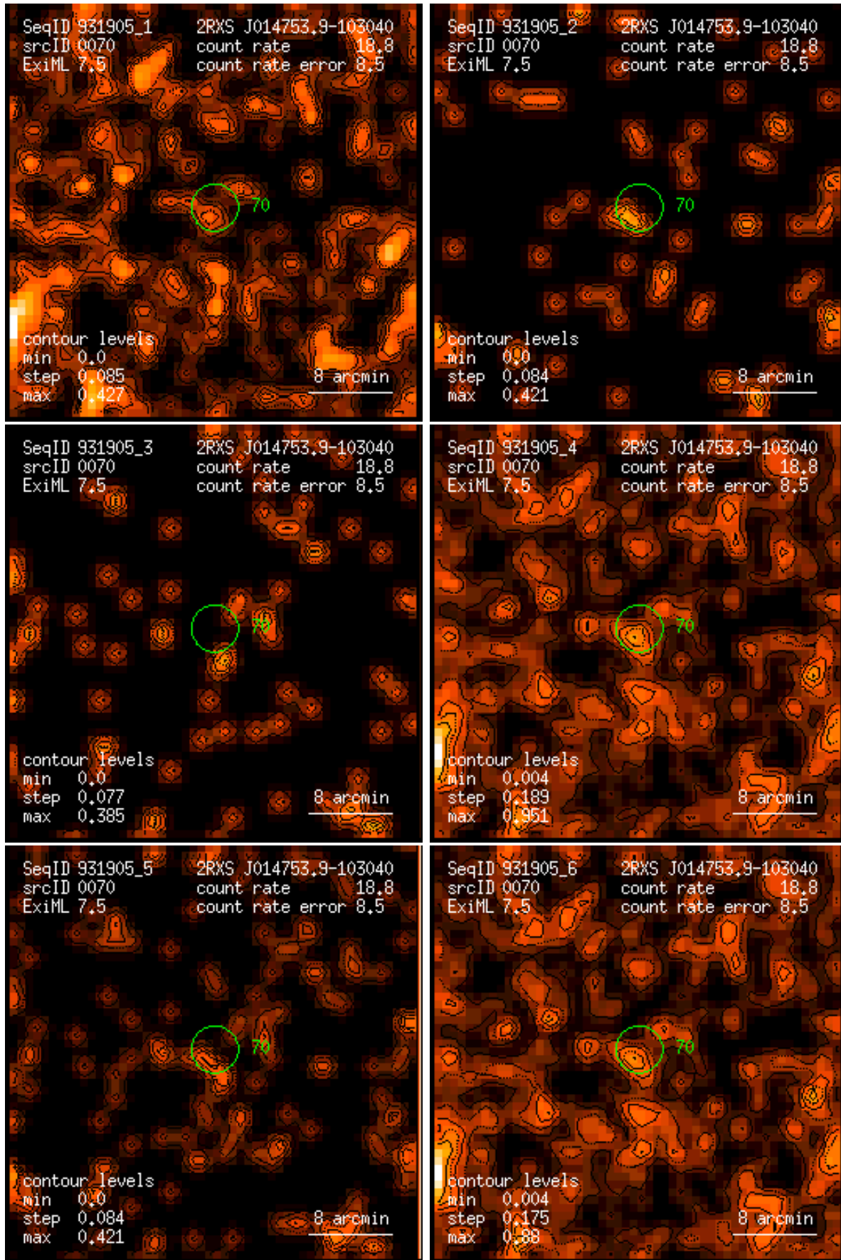
Figure 70: RASS 931905: detection 0070: band rate images, Gaussian filter: (1) PSPC channels 11 – 41, (2) 52 – 90, (3) 91 – 201, (4) 11 – 235, (5) 52 – 201, (6) 11 – 201. Broad band rates in counts/ks. Band rate contour levels in counts/ks/arcmin 2 .
