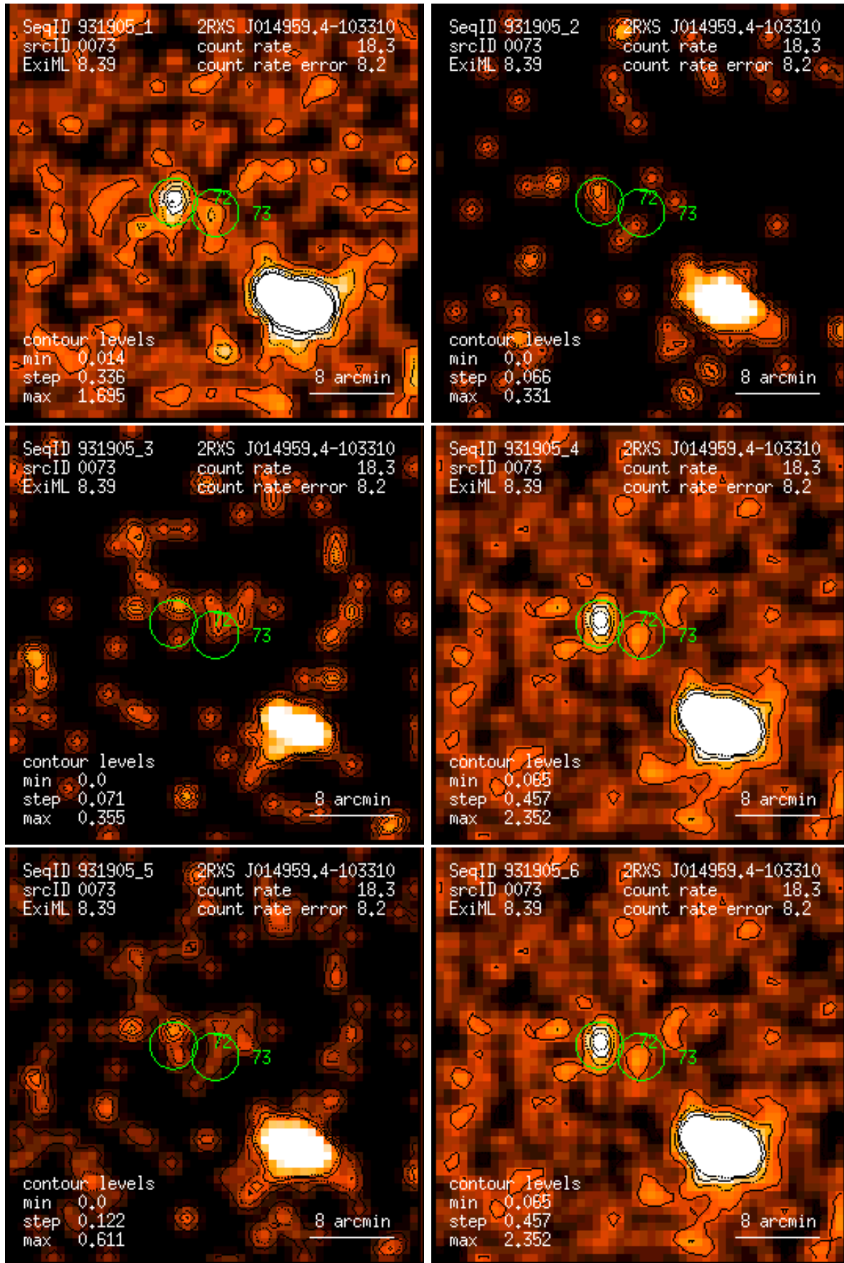
Figure 73: RASS 931905: detection 0073: band rate images, Gaussian filter: (1) PSPC channels 11 – 41, (2) 52 – 90, (3) 91 – 201, (4) 11 – 235, (5) 52 – 201, (6) 11 – 201. Broad band rates in counts/ks. Band rate contour levels in counts/ks/arcmin 2 .
