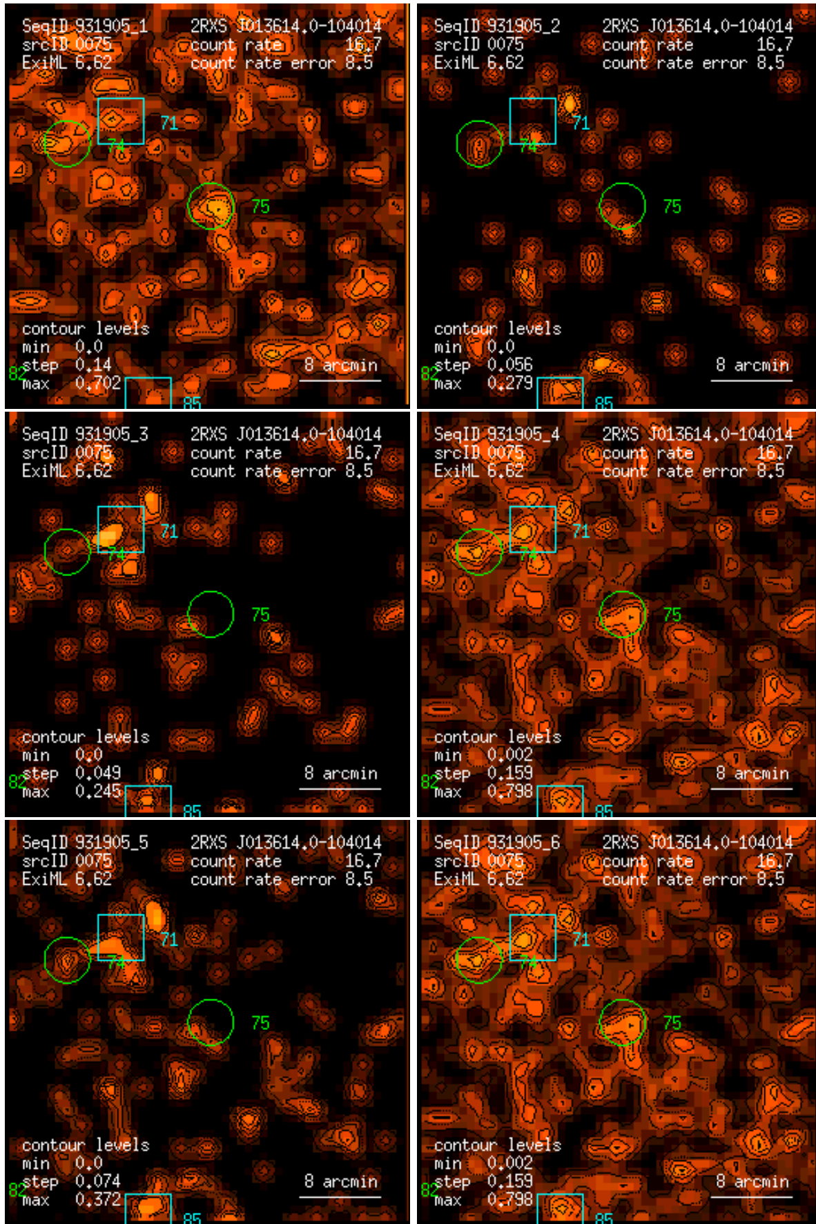
Figure 75: RASS 931905: detection 0075: band rate images, Gaussian filter: (1) PSPC channels 11 – 41, (2) 52 – 90, (3) 91 – 201, (4) 11 – 235, (5) 52 – 201, (6) 11 – 201. Broad band rates in counts/ks. Band rate contour levels in counts/ks/arcmin 2 .
