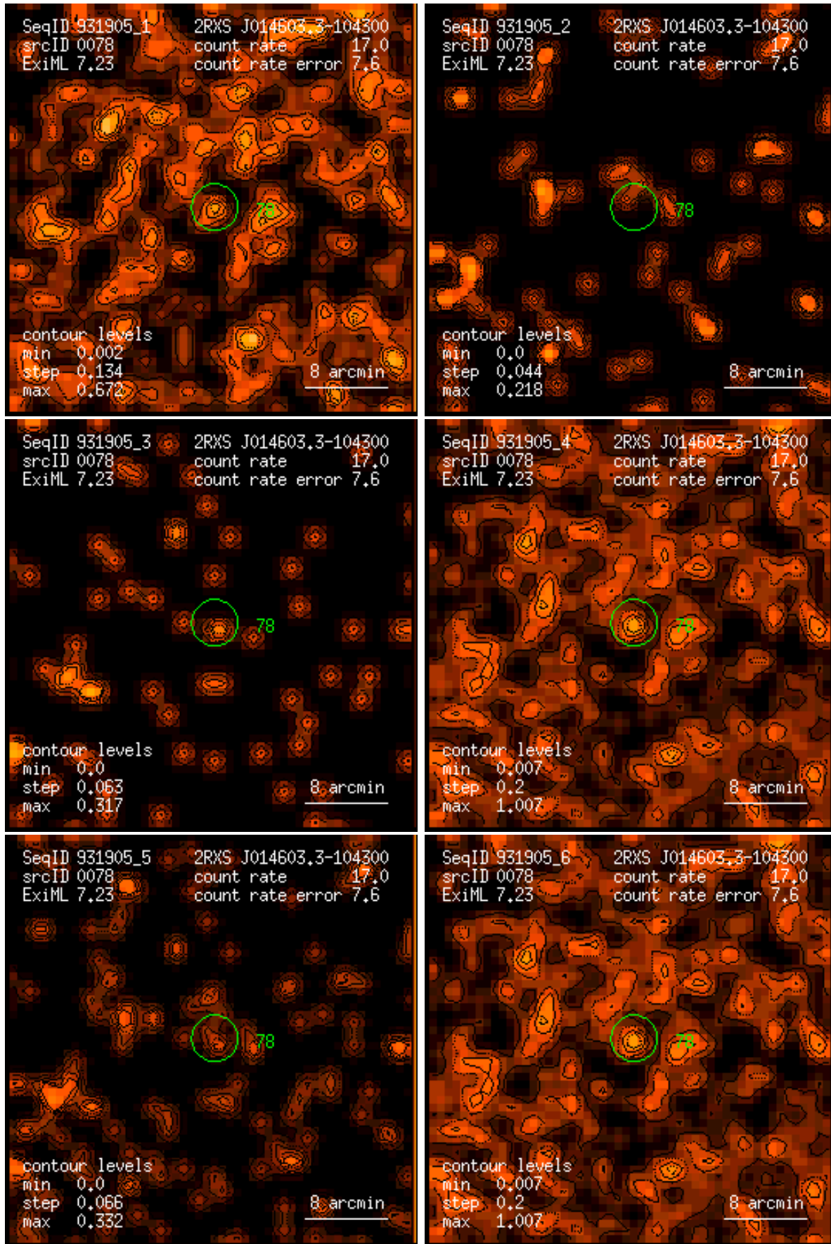
Figure 78: RASS 931905: detection 0078: band rate images, Gaussian filter: (1) PSPC channels 11 – 41, (2) 52 – 90, (3) 91 – 201, (4) 11 – 235, (5) 52 – 201, (6) 11 – 201. Broad band rates in counts/ks. Band rate contour levels in counts/ks/arcmin 2 .
