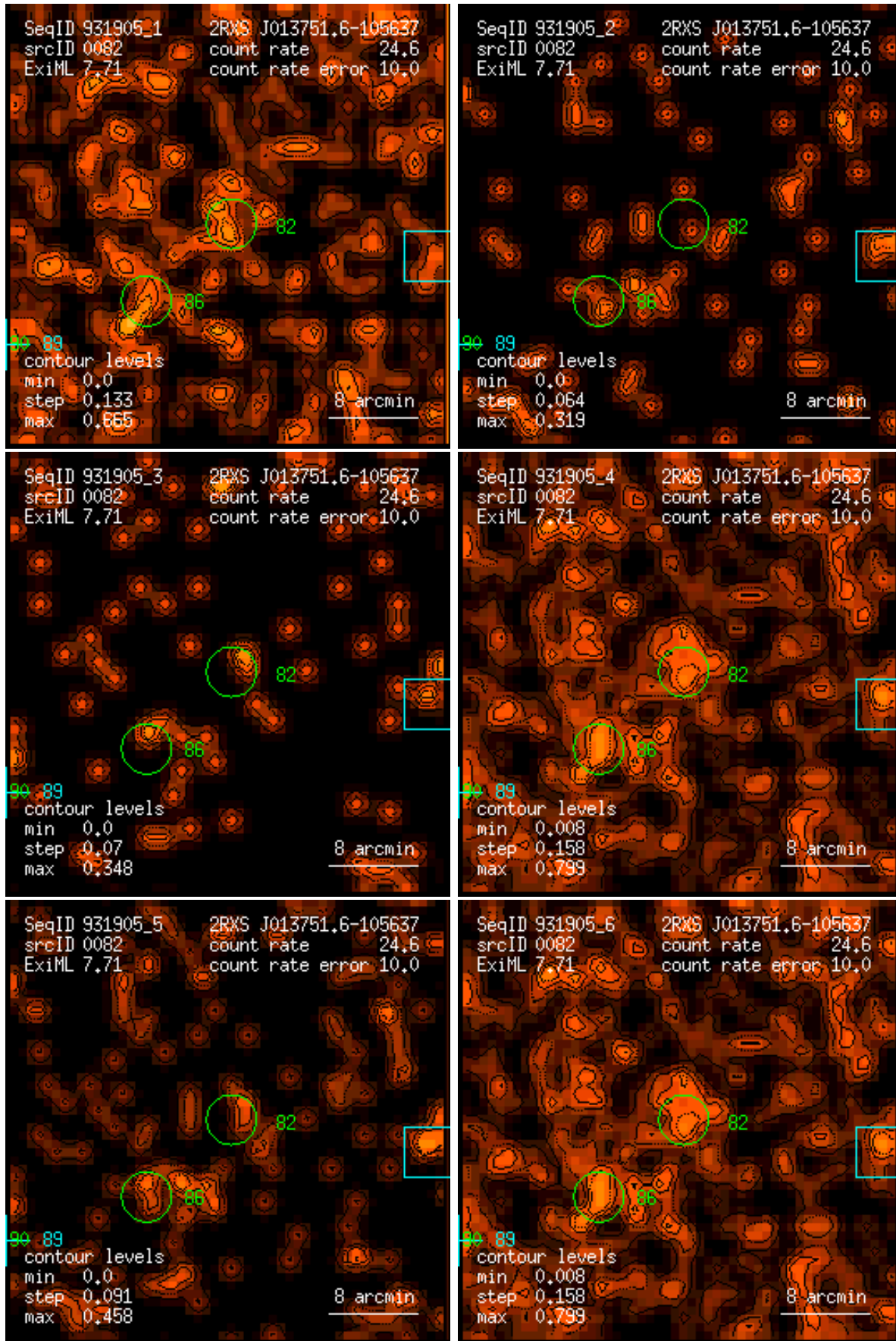
Figure 82: RASS 931905: detection 0082: band rate images, Gaussian filter: (1) PSPC channels 11 – 41, (2) 52 – 90, (3) 91 – 201, (4) 11 – 235, (5) 52 – 201, (6) 11 – 201. Broad band rates in counts/ks. Band rate contour levels in counts/ks/arcmin 2 .
