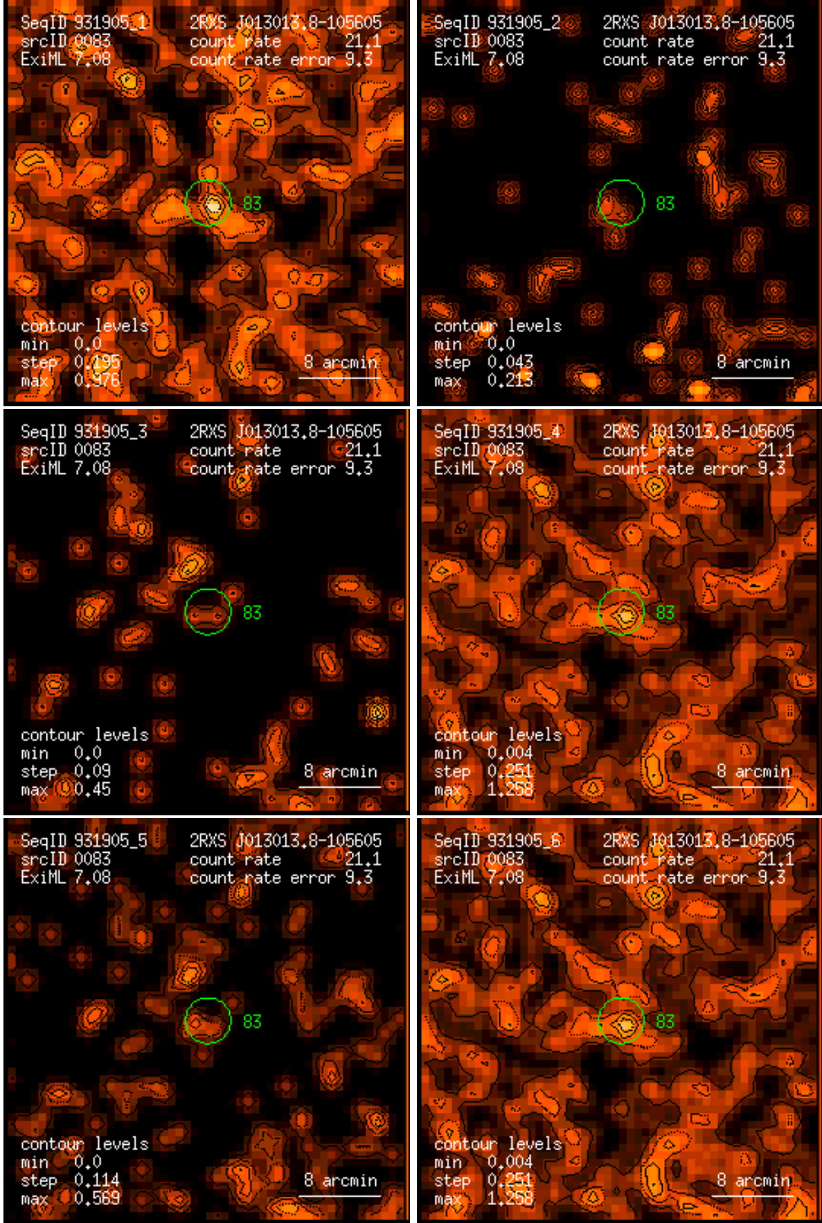
Figure 83: RASS 931905: detection 0083: band rate images, Gaussian filter: (1) PSPC channels 11 – 41, (2) 52 – 90, (3) 91 – 201, (4) 11 – 235, (5) 52 – 201, (6) 11 – 201. Broad band rates in counts/ks. Band rate contour levels in counts/ks/arcmin 2 .
