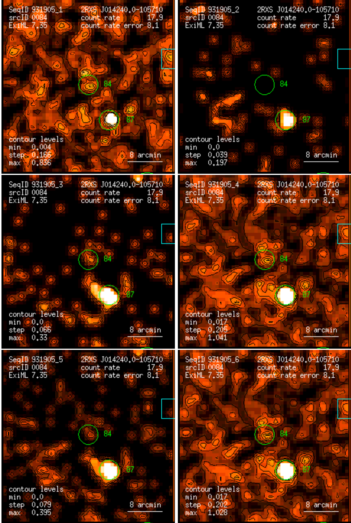
Figure 84: RASS 931905: detection 0084: band rate images, Gaussian filter: (1) PSPC channels 11 – 41, (2) 52 – 90, (3) 91 – 201, (4) 11 – 235, (5) 52 – 201, (6) 11 – 201. Broad band rates in counts/ks. Band rate contour levels in counts/ks/arcmin 2 .
