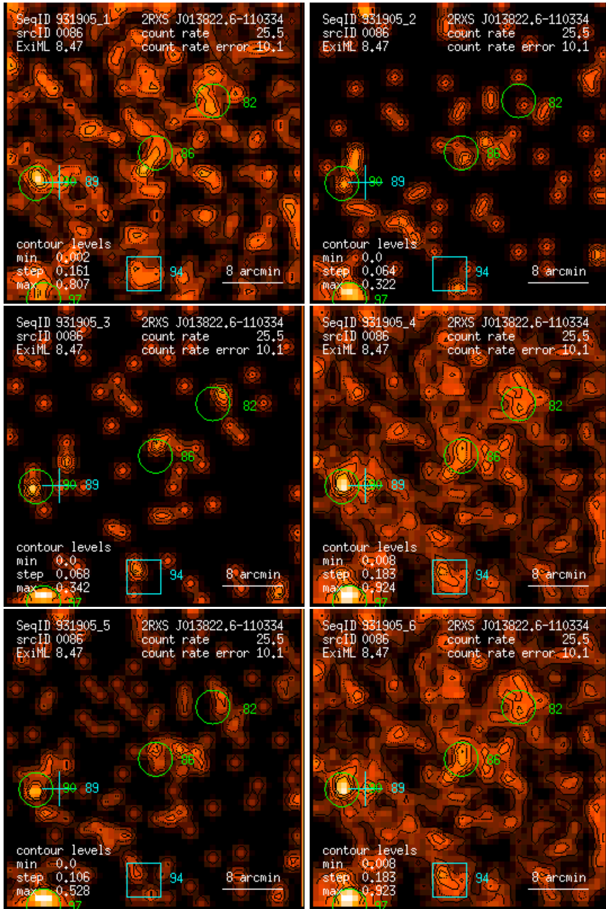
Figure 86: RASS 931905: detection 0086: band rate images, Gaussian filter: (1) PSPC channels 11 – 41, (2) 52 – 90, (3) 91 – 201, (4) 11 – 235, (5) 52 – 201, (6) 11 – 201. Broad band rates in counts/ks. Band rate contour levels in counts/ks/arcmin 2 .
