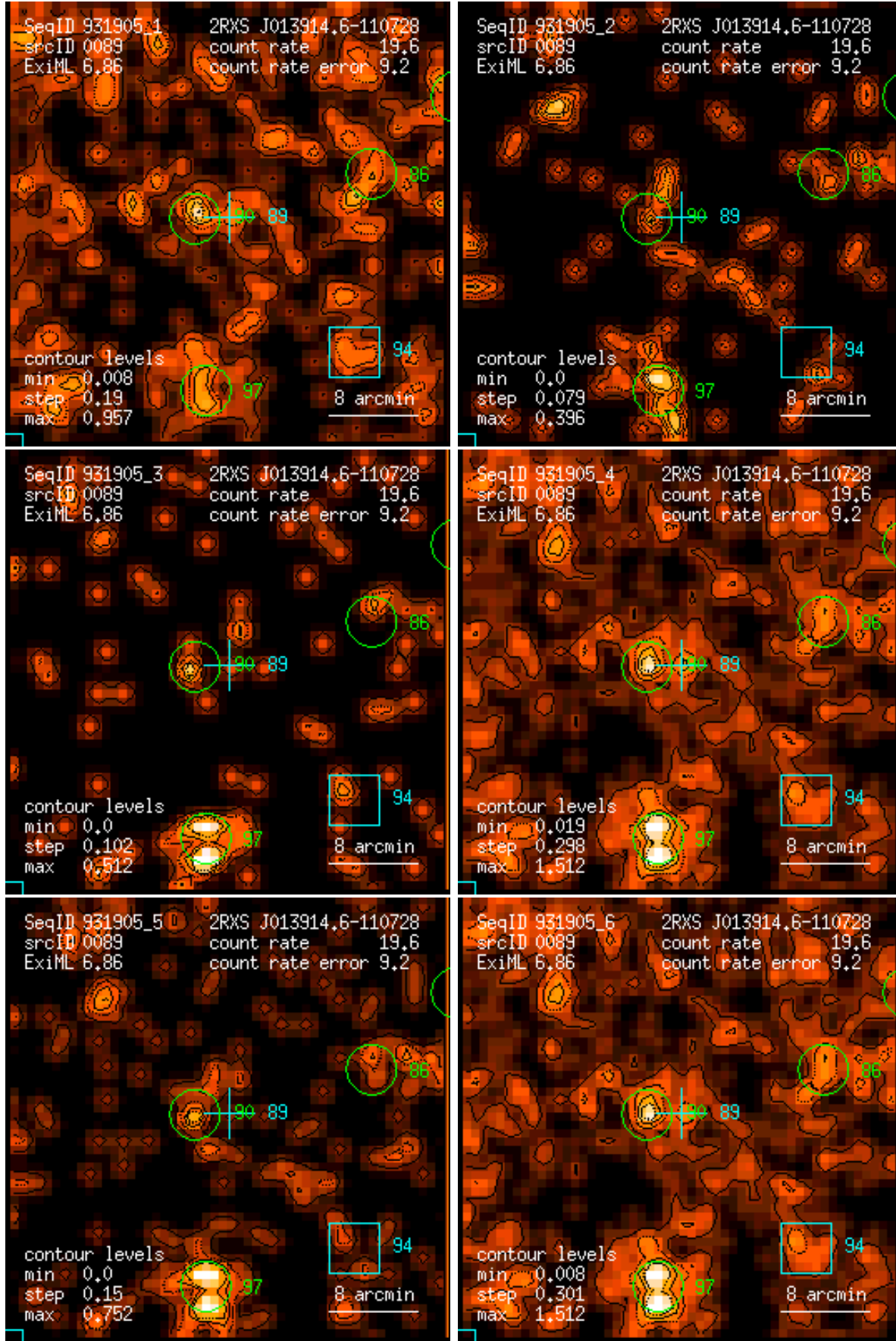
Figure 89: RASS 931905: detection 0089: band rate images, Gaussian filter: (1) PSPC channels 11 – 41, (2) 52 – 90, (3) 91 – 201, (4) 11 – 235, (5) 52 – 201, (6) 11 – 201. Broad band rates in counts/ks. Band rate contour levels in counts/ks/arcmin 2 .
