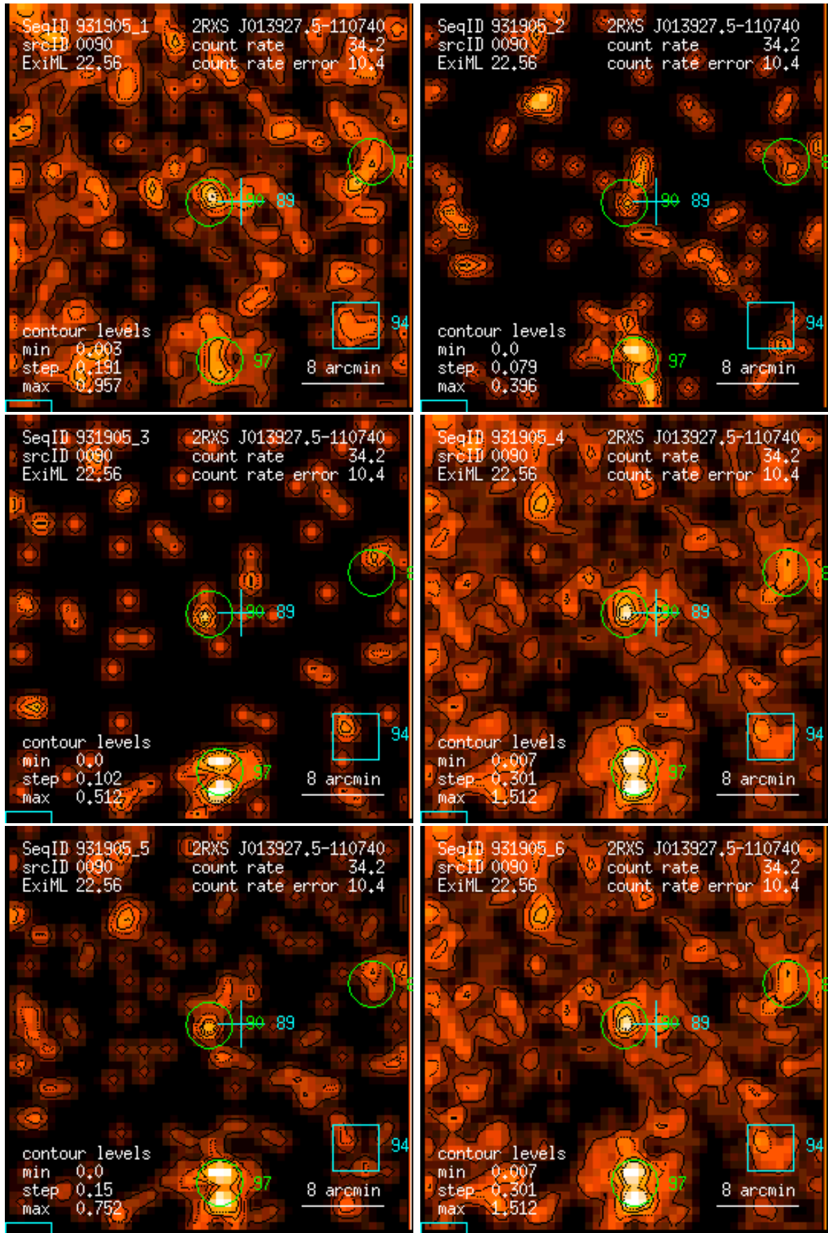
Figure 90: RASS 931905: detection 0090: band rate images, Gaussian filter: (1) PSPC channels 11 – 41, (2) 52 – 90, (3) 91 – 201, (4) 11 – 235, (5) 52 – 201, (6) 11 – 201. Broad band rates in counts/ks. Band rate contour levels in counts/ks/arcmin 2 .
