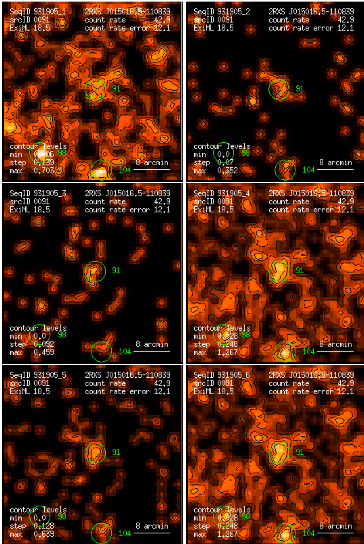
Figure 91: RASS 931905: detection 0091: band rate images, Gaussian filter: (1) PSPC channels 11 – 41, (2) 52 – 90, (3) 91 – 201, (4) 11 – 235, (5) 52 – 201, (6) 11 – 201. Broad band rates in counts/ks. Band rate contour levels in counts/ks/arcmin 2 .
