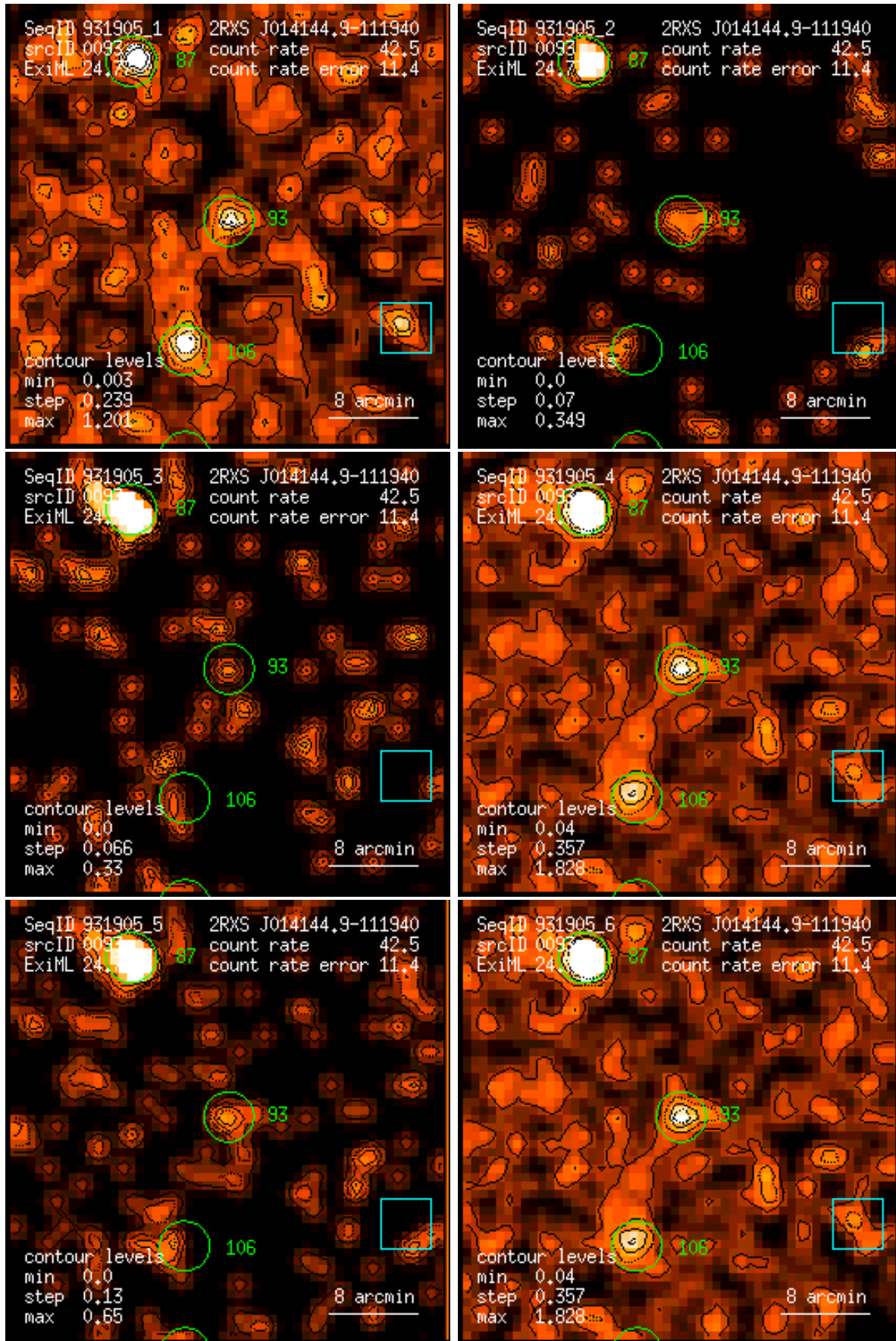
Figure 93: RASS 931905: detection 0093: band rate images, Gaussian filter: (1) PSPC channels 11 – 41, (2) 52 – 90, (3) 91 – 201, (4) 11 – 235, (5) 52 – 201, (6) 11 – 201. Broad band rates in counts/ks. Band rate contour levels in counts/ks/arcmin 2 .
