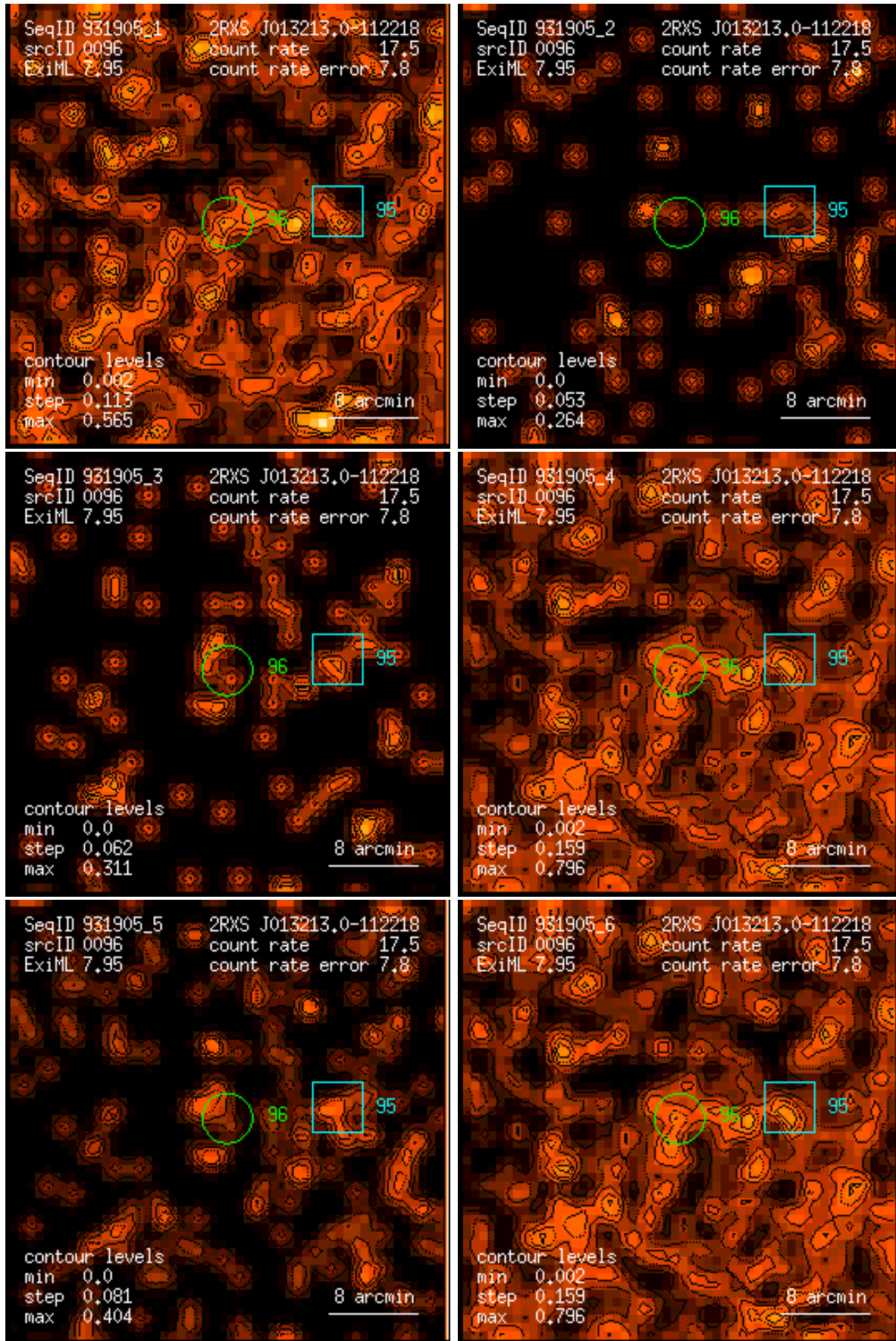
Figure 96: RASS 931905: detection 0096: band rate images, Gaussian filter: (1) PSPC channels 11 – 41, (2) 52 – 90, (3) 91 – 201, (4) 11 – 235, (5) 52 – 201, (6) 11 – 201. Broad band rates in counts/ks. Band rate contour levels in counts/ks/arcmin 2 .
