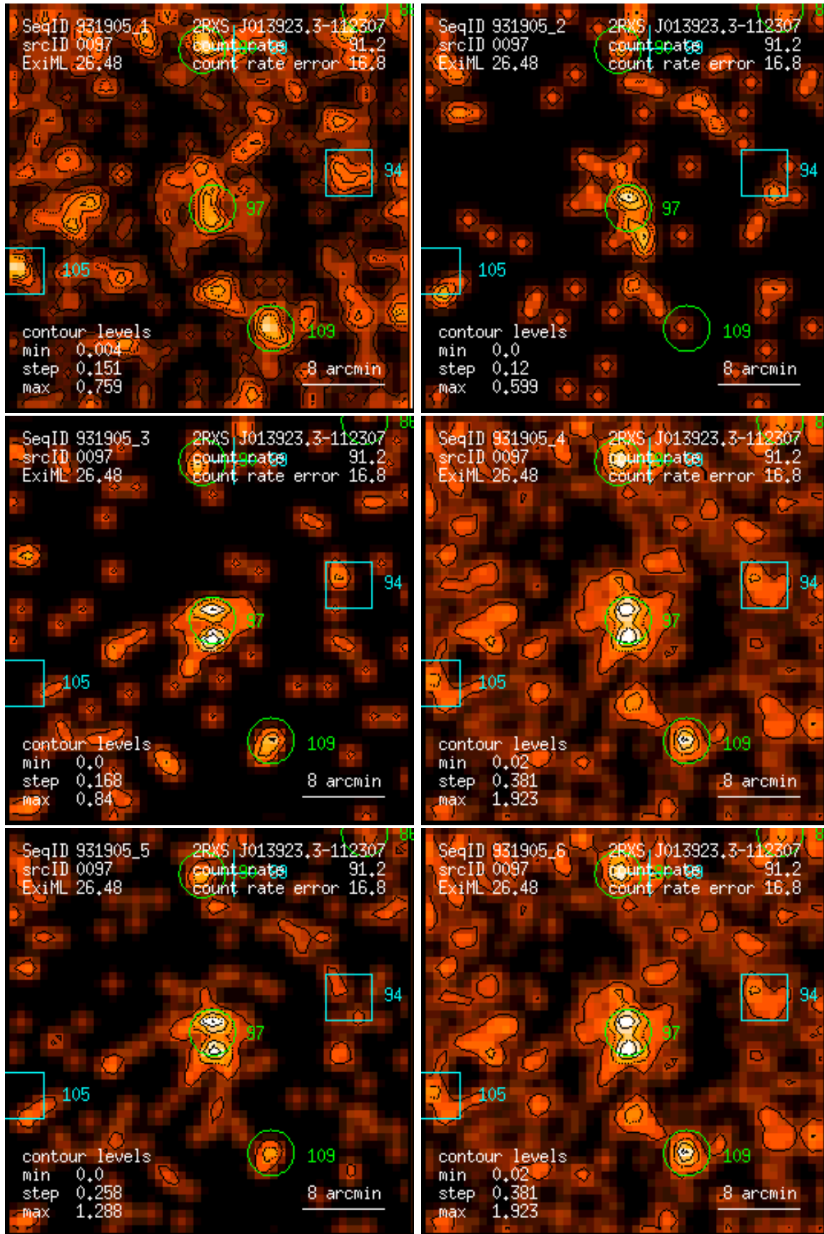
Figure 97: RASS 931905: detection 0097: band rate images, Gaussian filter: (1) PSPC channels 11 – 41, (2) 52 – 90, (3) 91 – 201, (4) 11 – 235, (5) 52 – 201, (6) 11 – 201. Broad band rates in counts/ks. Band rate contour levels in counts/ks/arcmin 2 .
