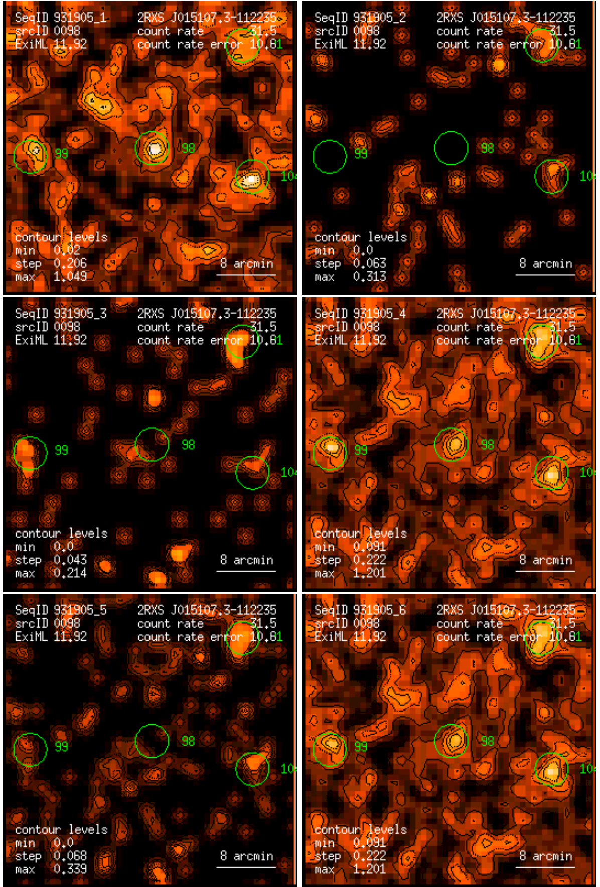
Figure 98: RASS 931905: detection 0098: band rate images, Gaussian filter: (1) PSPC channels 11 – 41, (2) 52 – 90, (3) 91 – 201, (4) 11 – 235, (5) 52 – 201, (6) 11 – 201. Broad band rates in counts/ks. Band rate contour levels in counts/ks/arcmin 2 .
