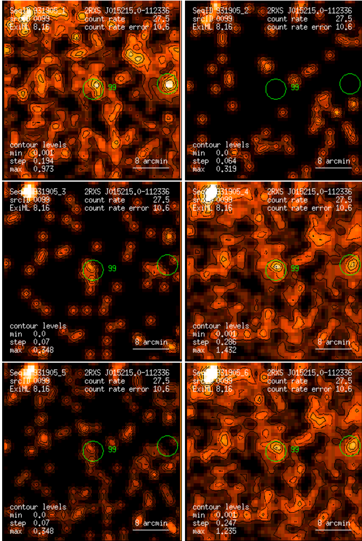
Figure 99: RASS 931905: detection 0099: band rate images, Gaussian filter: (1) PSPC channels 11 – 41, (2) 52 – 90, (3) 91 – 201, (4) 11 – 235, (5) 52 – 201, (6) 11 – 201. Broad band rates in counts/ks. Band rate contour levels in counts/ks/arcmin 2 .
