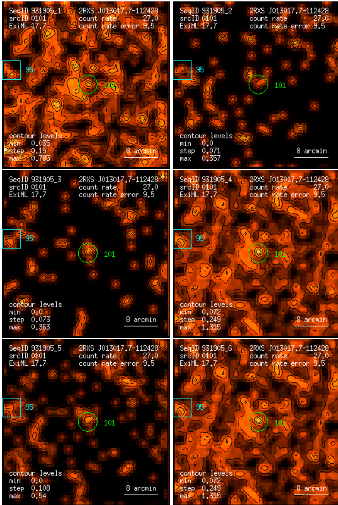
Figure 101: RASS 931905: detection 0101: band rate images, Gaussian filter: (1) PSPC channels 11 – 41, (2) 52 – 90, (3) 91 – 201, (4) 11 – 235, (5) 52 – 201, (6) 11 – 201. Broad band rates in counts/ks. Band rate contour levels in counts/ks/arcmin 2 .
