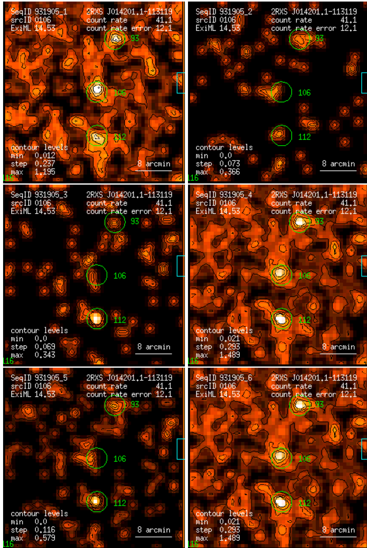
Figure 106: RASS 931905: detection 0106: band rate images, Gaussian filter: (1) PSPC channels 11 – 41, (2) 52 – 90, (3) 91 – 201, (4) 11 – 235, (5) 52 – 201, (6) 11 – 201. Broad band rates in counts/ks. Band rate contour levels in counts/ks/arcmin 2 .
