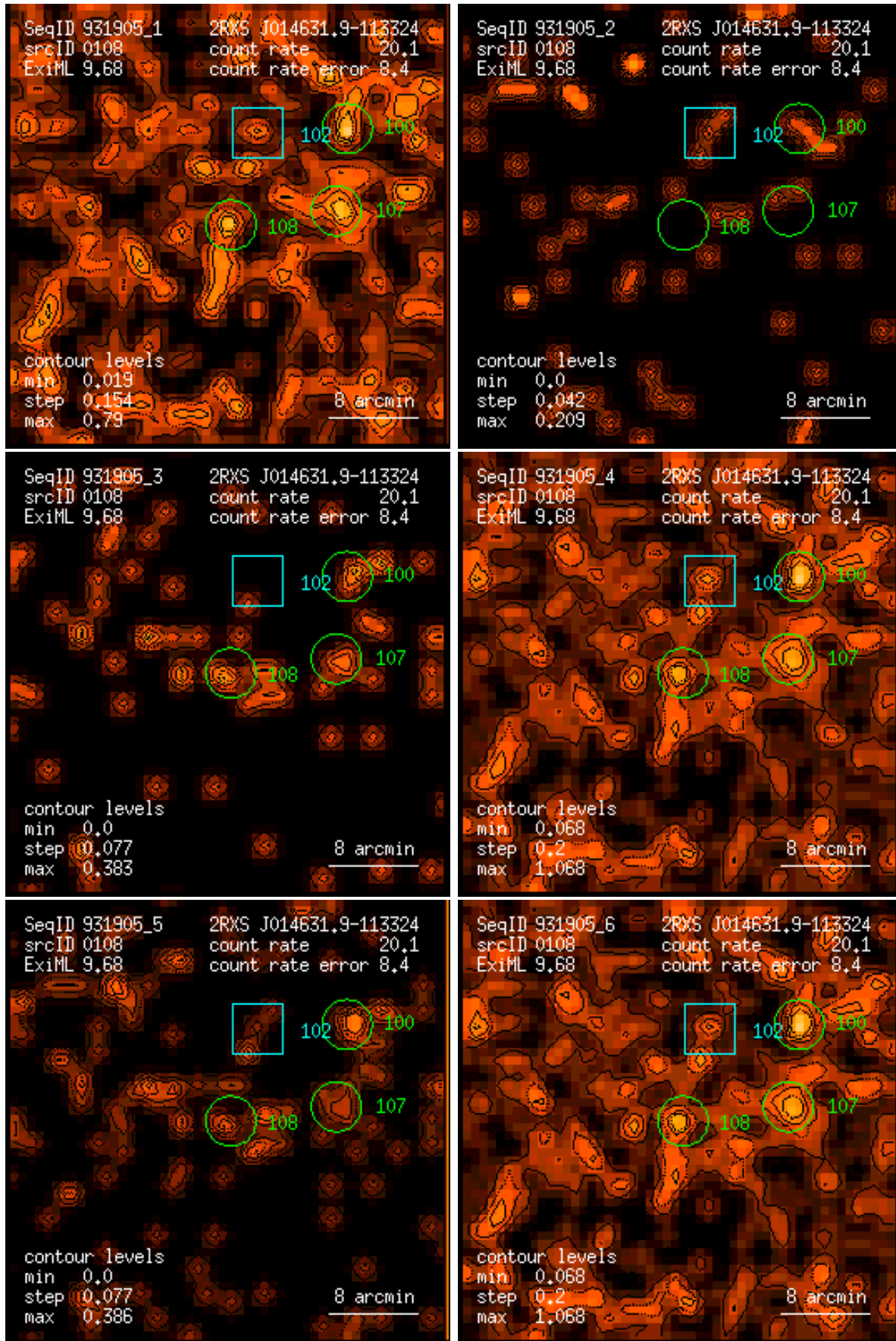
Figure 108: RASS 931905: detection 0108: band rate images, Gaussian filter: (1) PSPC channels 11 – 41, (2) 52 – 90, (3) 91 – 201, (4) 11 – 235, (5) 52 – 201, (6) 11 – 201. Broad band rates in counts/ks. Band rate contour levels in counts/ks/arcmin 2 .
