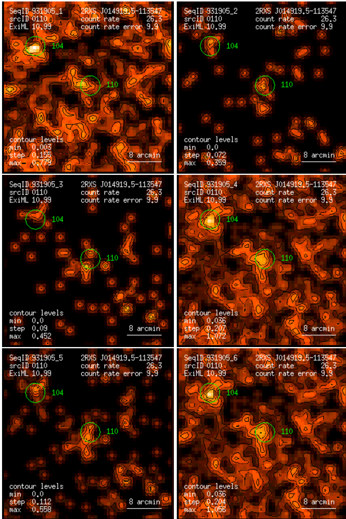
Figure 110: RASS 931905: detection 0110: band rate images, Gaussian filter: (1) PSPC channels 11 – 41, (2) 52 – 90, (3) 91 – 201, (4) 11 – 235, (5) 52 – 201, (6) 11 – 201. Broad band rates in counts/ks. Band rate contour levels in counts/ks/arcmin 2 .
