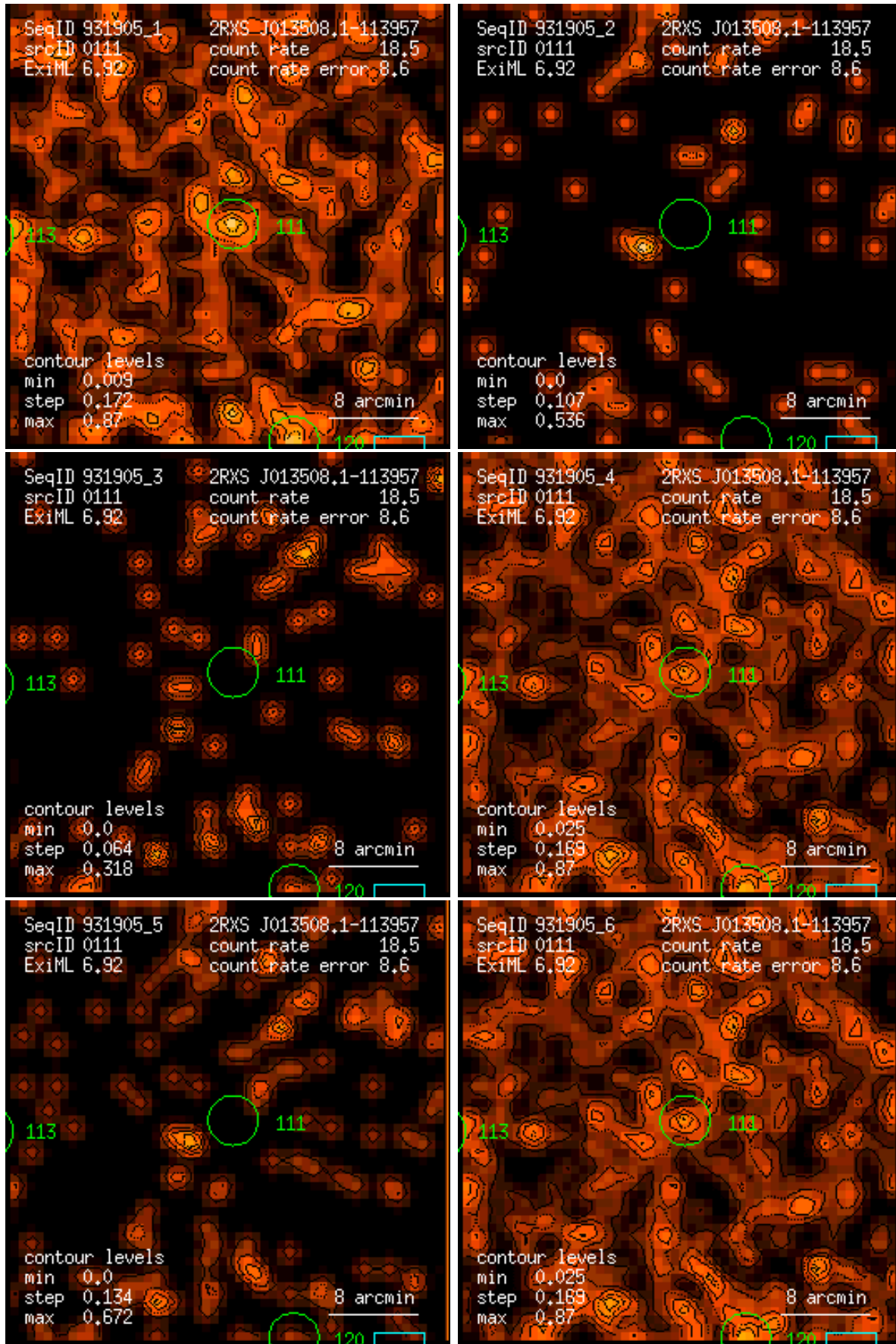
Figure 111: RASS 931905: detection 0111: band rate images, Gaussian filter: (1) PSPC channels 11 – 41, (2) 52 – 90, (3) 91 – 201, (4) 11 – 235, (5) 52 – 201, (6) 11 – 201. Broad band rates in counts/ks. Band rate contour levels in counts/ks/arcmin 2 .
