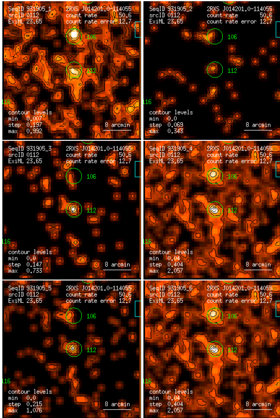
Figure 112: RASS 931905: detection 0112: band rate images, Gaussian filter: (1) PSPC channels 11 – 41, (2) 52 – 90, (3) 91 – 201, (4) 11 – 235, (5) 52 – 201, (6) 11 – 201. Broad band rates in counts/ks. Band rate contour levels in counts/ks/arcmin 2 .
