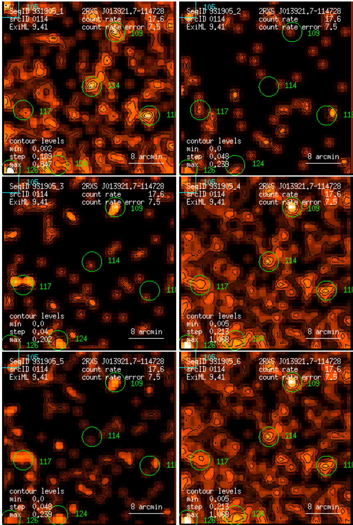
Figure 114: RASS 931905: detection 0114: band rate images, Gaussian filter: (1) PSPC channels 11 – 41, (2) 52 – 90, (3) 91 – 201, (4) 11 – 235, (5) 52 – 201, (6) 11 – 201. Broad band rates in counts/ks. Band rate contour levels in counts/ks/arcmin 2 .
