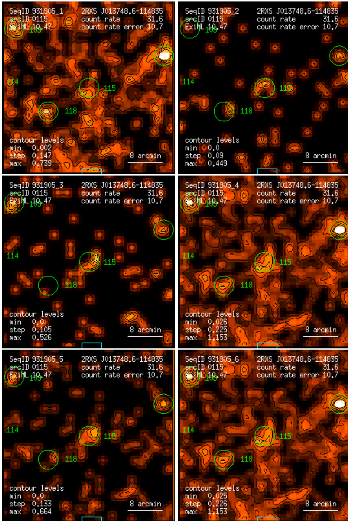
Figure 115: RASS 931905: detection 0115: band rate images, Gaussian filter: (1) PSPC channels 11 – 41, (2) 52 – 90, (3) 91 – 201, (4) 11 – 235, (5) 52 – 201, (6) 11 – 201. Broad band rates in counts/ks. Band rate contour levels in counts/ks/arcmin 2 .
