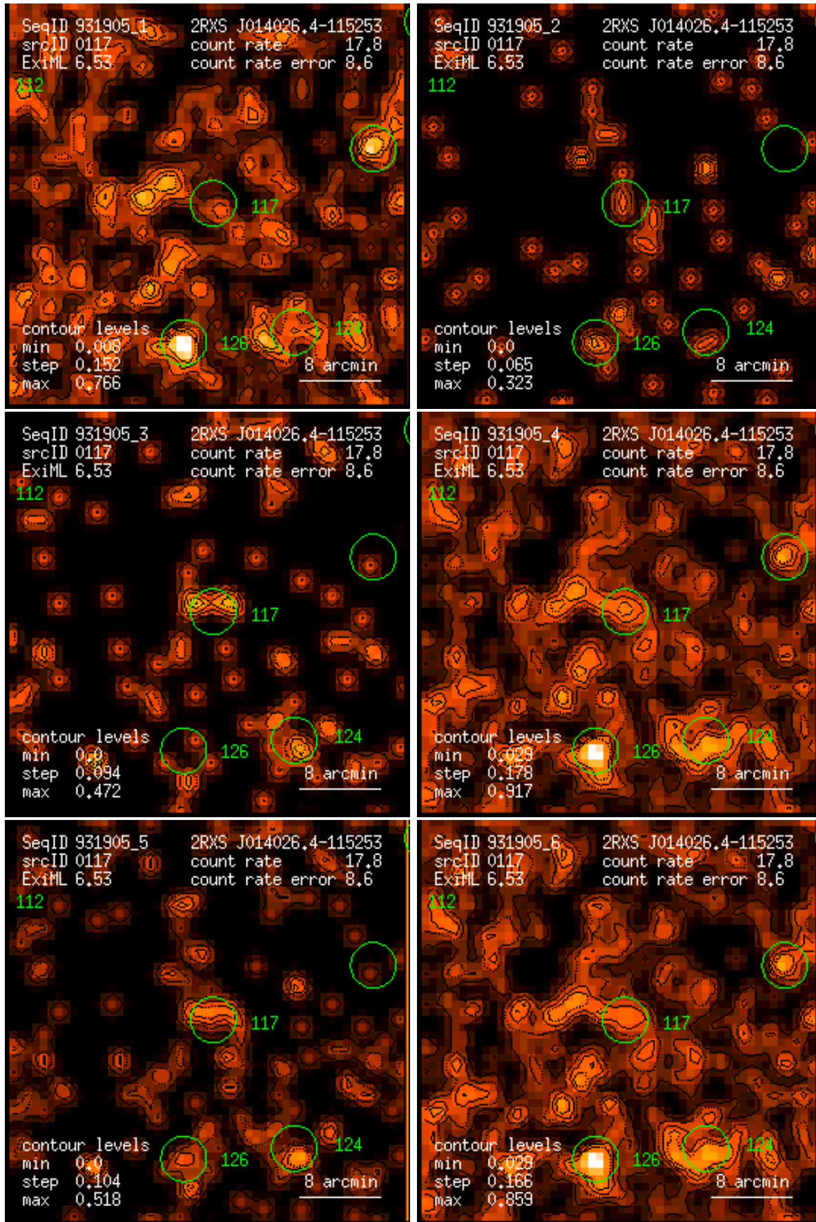
Figure 117: RASS 931905: detection 0117: band rate images, Gaussian filter: (1) PSPC channels 11 – 41, (2) 52 – 90, (3) 91 – 201, (4) 11 – 235, (5) 52 – 201, (6) 11 – 201. Broad band rates in counts/ks. Band rate contour levels in counts/ks/arcmin 2 .
