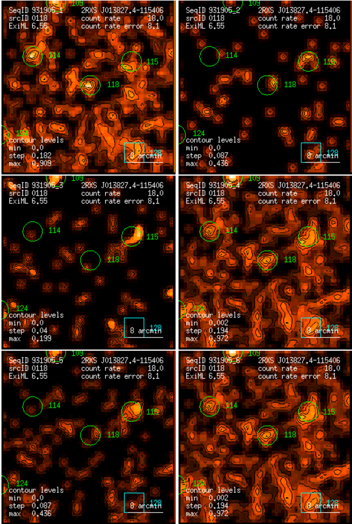
Figure 118: RASS 931905: detection 0118: band rate images, Gaussian filter: (1) PSPC channels 11 – 41, (2) 52 – 90, (3) 91 – 201, (4) 11 – 235, (5) 52 – 201, (6) 11 – 201. Broad band rates in counts/ks. Band rate contour levels in counts/ks/arcmin 2 .
