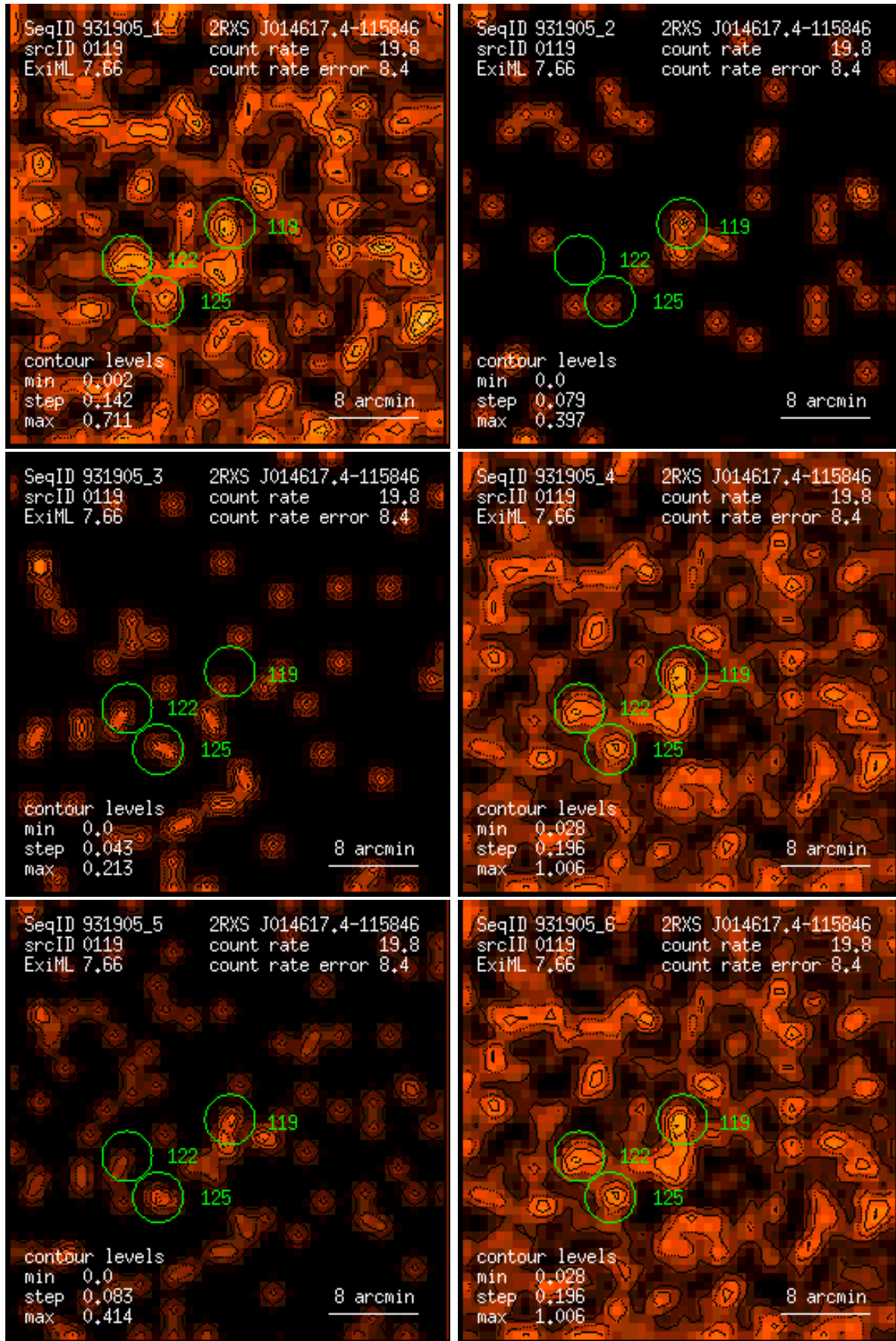
Figure 119: RASS 931905: detection 0119: band rate images, Gaussian filter: (1) PSPC channels 11 – 41, (2) 52 – 90, (3) 91 – 201, (4) 11 – 235, (5) 52 – 201, (6) 11 – 201. Broad band rates in counts/ks. Band rate contour levels in counts/ks/arcmin 2 .
