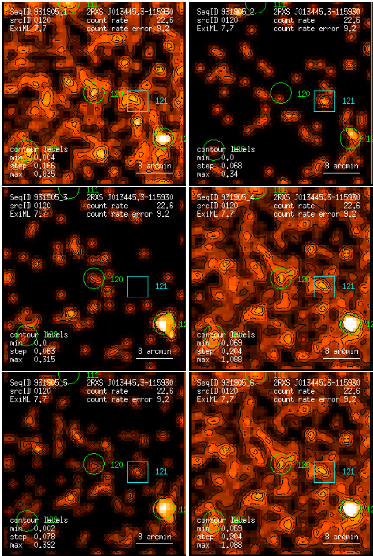
Figure 120: RASS 931905: detection 0120: band rate images, Gaussian filter: (1) PSPC channels 11 – 41, (2) 52 – 90, (3) 91 – 201, (4) 11 – 235, (5) 52 – 201, (6) 11 – 201. Broad band rates in counts/ks. Band rate contour levels in counts/ks/arcmin 2 .
