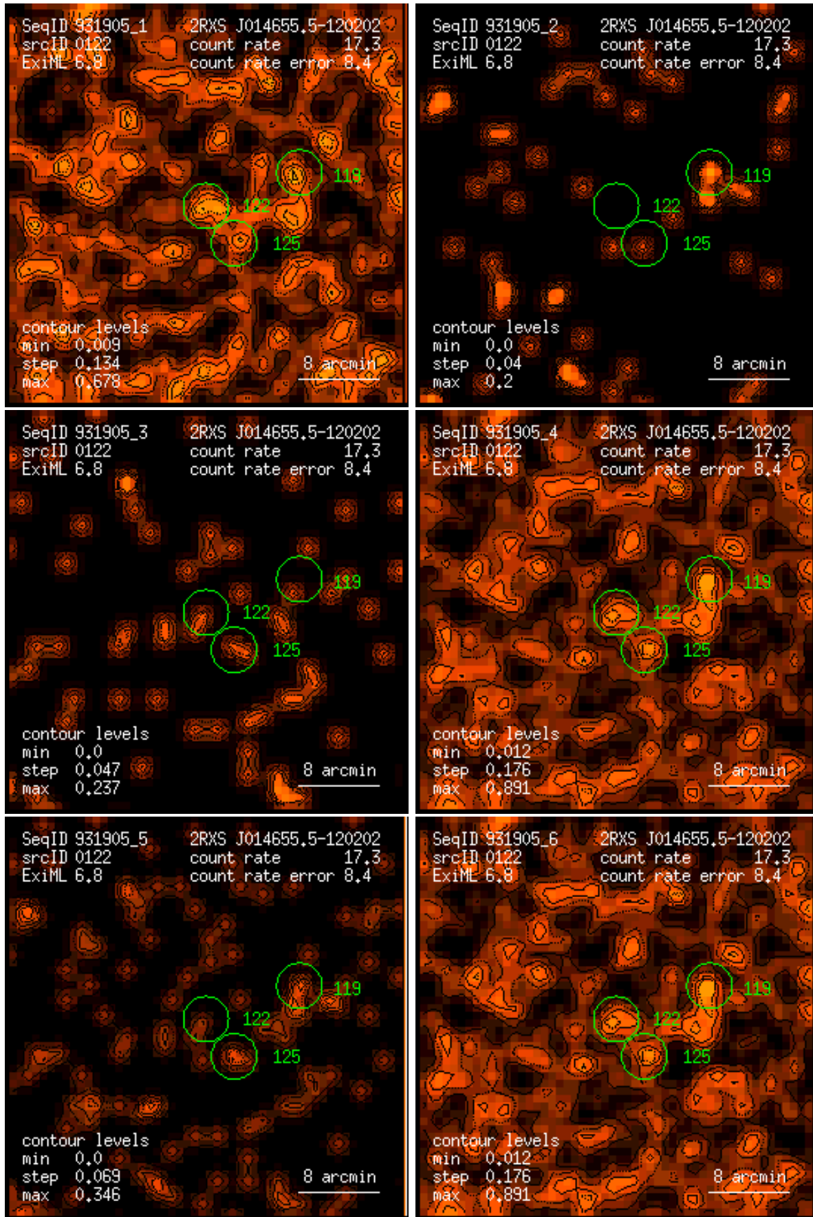
Figure 122: RASS 931905: detection 0122: band rate images, Gaussian filter: (1) PSPC channels 11 – 41, (2) 52 – 90, (3) 91 – 201, (4) 11 – 235, (5) 52 – 201, (6) 11 – 201. Broad band rates in counts/ks. Band rate contour levels in counts/ks/arcmin 2 .
