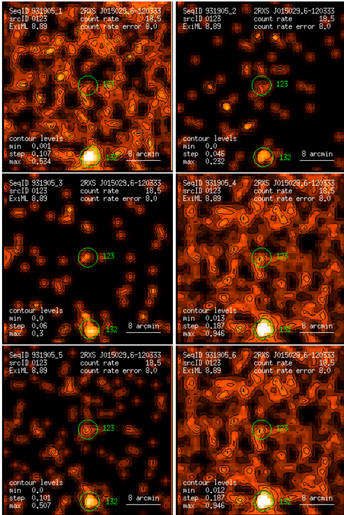
Figure 123: RASS 931905: detection 0123: band rate images, Gaussian filter: (1) PSPC channels 11 – 41, (2) 52 – 90, (3) 91 – 201, (4) 11 – 235, (5) 52 – 201, (6) 11 – 201. Broad band rates in counts/ks. Band rate contour levels in counts/ks/arcmin 2 .
