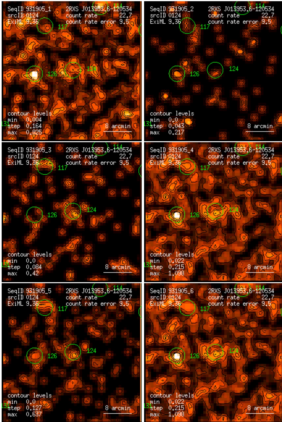
Figure 124: RASS 931905: detection 0124: band rate images, Gaussian filter: (1) PSPC channels 11 – 41, (2) 52 – 90, (3) 91 – 201, (4) 11 – 235, (5) 52 – 201, (6) 11 – 201. Broad band rates in counts/ks. Band rate contour levels in counts/ks/arcmin 2 .
