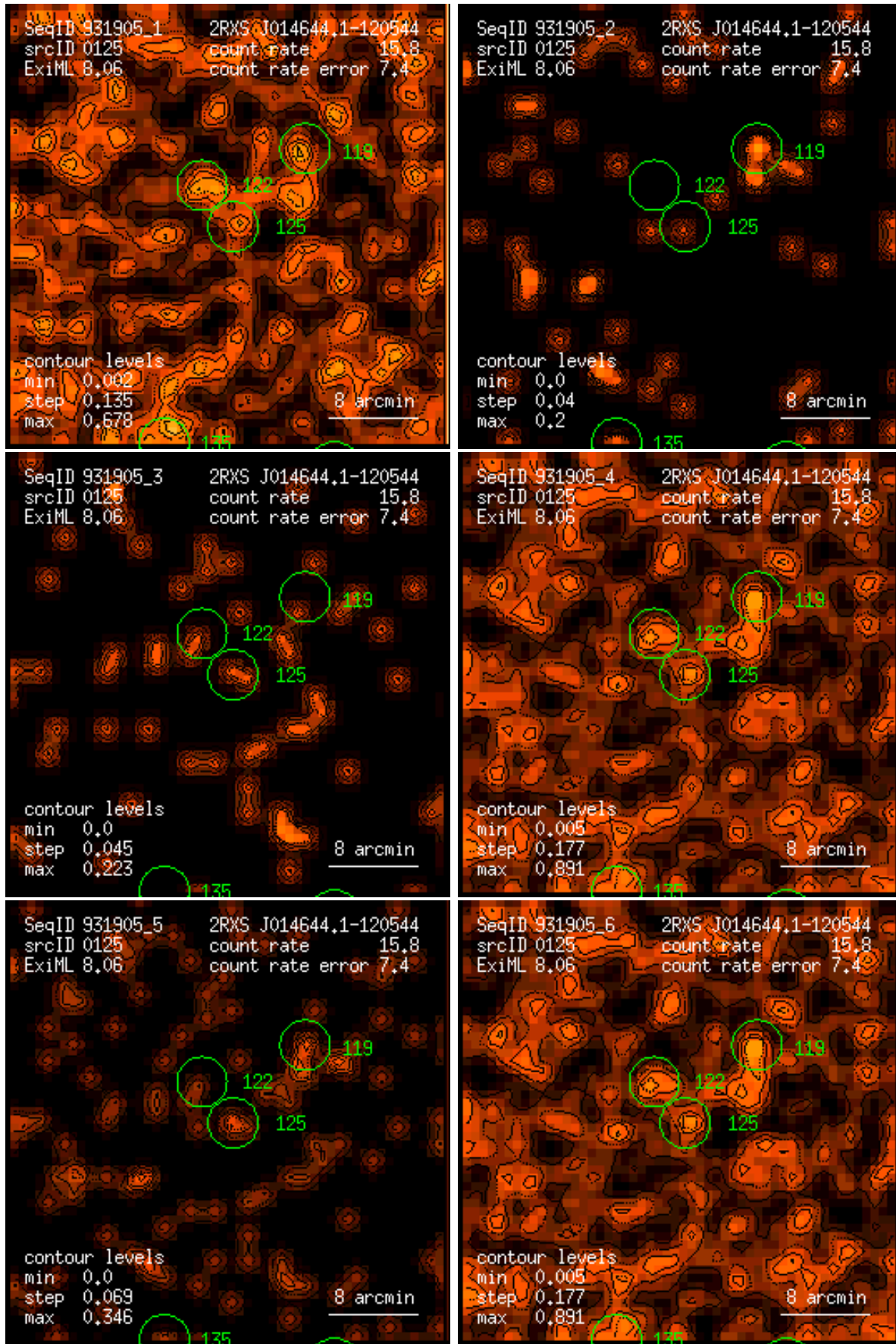
Figure 125: RASS 931905: detection 0125: band rate images, Gaussian filter: (1) PSPC channels 11 – 41, (2) 52 – 90, (3) 91 – 201, (4) 11 – 235, (5) 52 – 201, (6) 11 – 201. Broad band rates in counts/ks. Band rate contour levels in counts/ks/arcmin 2 .
