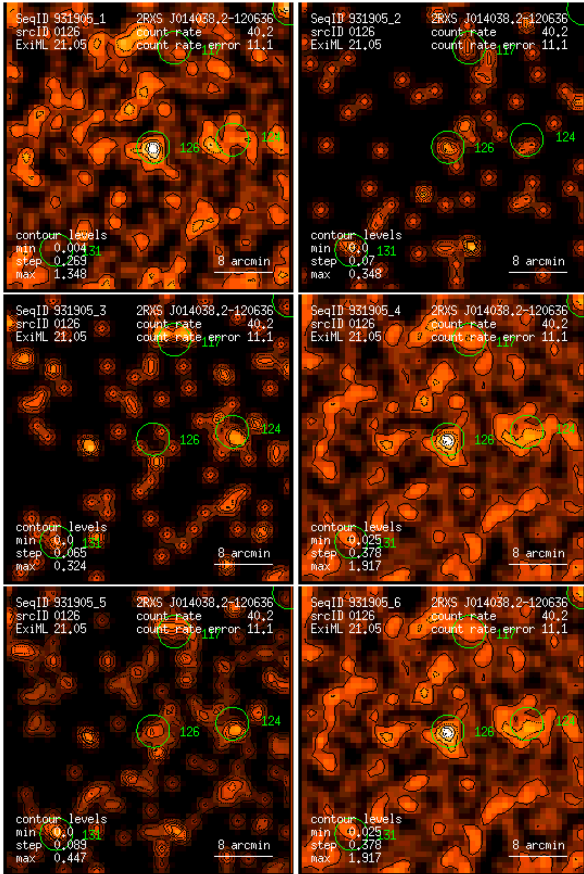
Figure 126: RASS 931905: detection 0126: band rate images, Gaussian filter: (1) PSPC channels 11 – 41, (2) 52 – 90, (3) 91 – 201, (4) 11 – 235, (5) 52 – 201, (6) 11 – 201. Broad band rates in counts/ks. Band rate contour levels in counts/ks/arcmin 2 .
