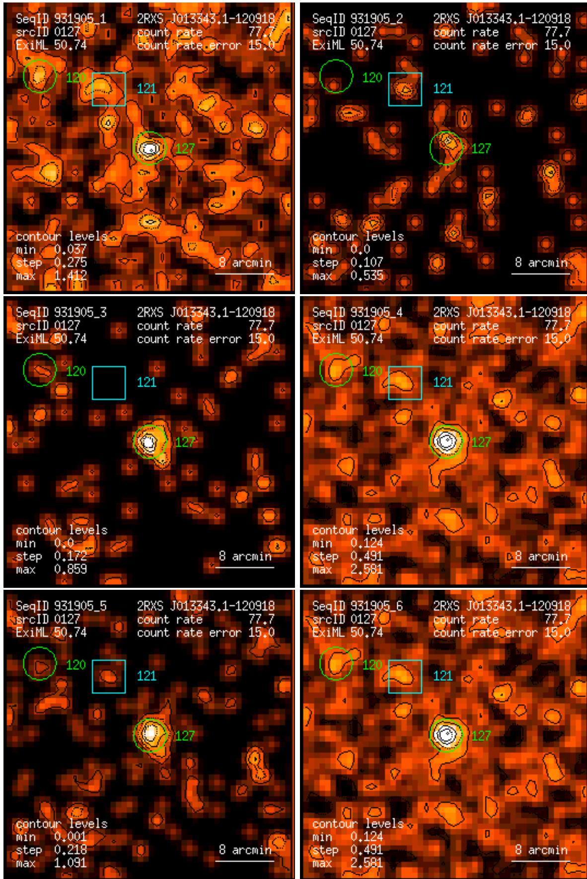
Figure 127: RASS 931905: detection 0127: band rate images, Gaussian filter: (1) PSPC channels 11 – 41, (2) 52 – 90, (3) 91 – 201, (4) 11 – 235, (5) 52 – 201, (6) 11 – 201. Broad band rates in counts/ks. Band rate contour levels in counts/ks/arcmin 2 .
