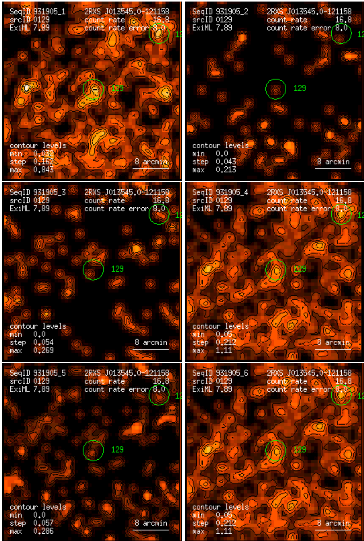
Figure 129: RASS 931905: detection 0129: band rate images, Gaussian filter: (1) PSPC channels 11 – 41, (2) 52 – 90, (3) 91 – 201, (4) 11 – 235, (5) 52 – 201, (6) 11 – 201. Broad band rates in counts/ks. Band rate contour levels in counts/ks/arcmin 2 .
