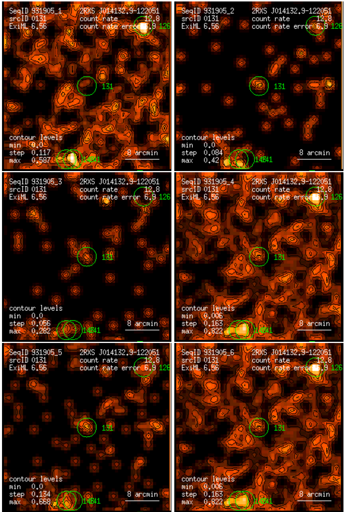
Figure 131: RASS 931905: detection 0131: band rate images, Gaussian filter: (1) PSPC channels 11 – 41, (2) 52 – 90, (3) 91 – 201, (4) 11 – 235, (5) 52 – 201, (6) 11 – 201. Broad band rates in counts/ks. Band rate contour levels in counts/ks/arcmin 2 .
