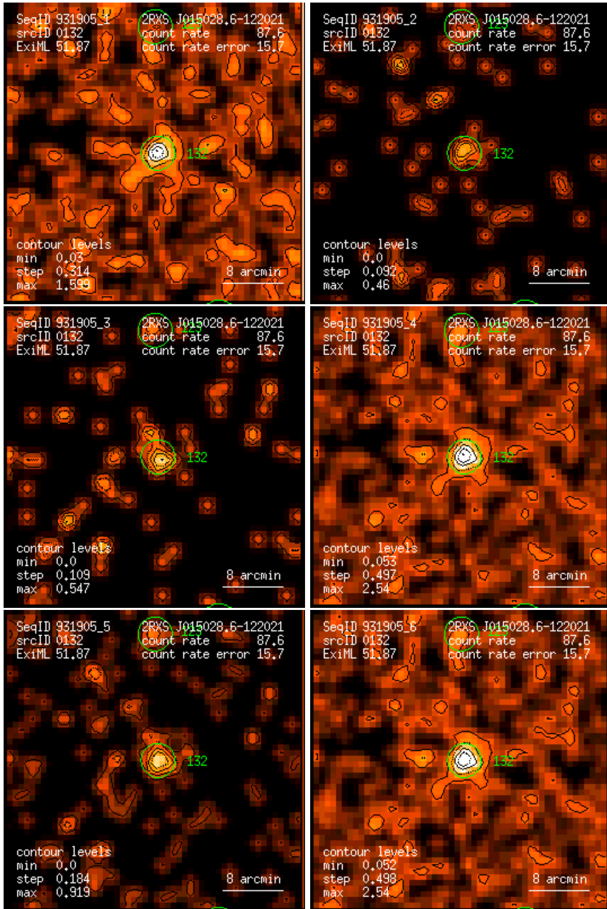
Figure 132: RASS 931905: detection 0132: band rate images, Gaussian filter: (1) PSPC channels 11 – 41, (2) 52 – 90, (3) 91 – 201, (4) 11 – 235, (5) 52 – 201, (6) 11 – 201. Broad band rates in counts/ks. Band rate contour levels in counts/ks/arcmin 2 .
