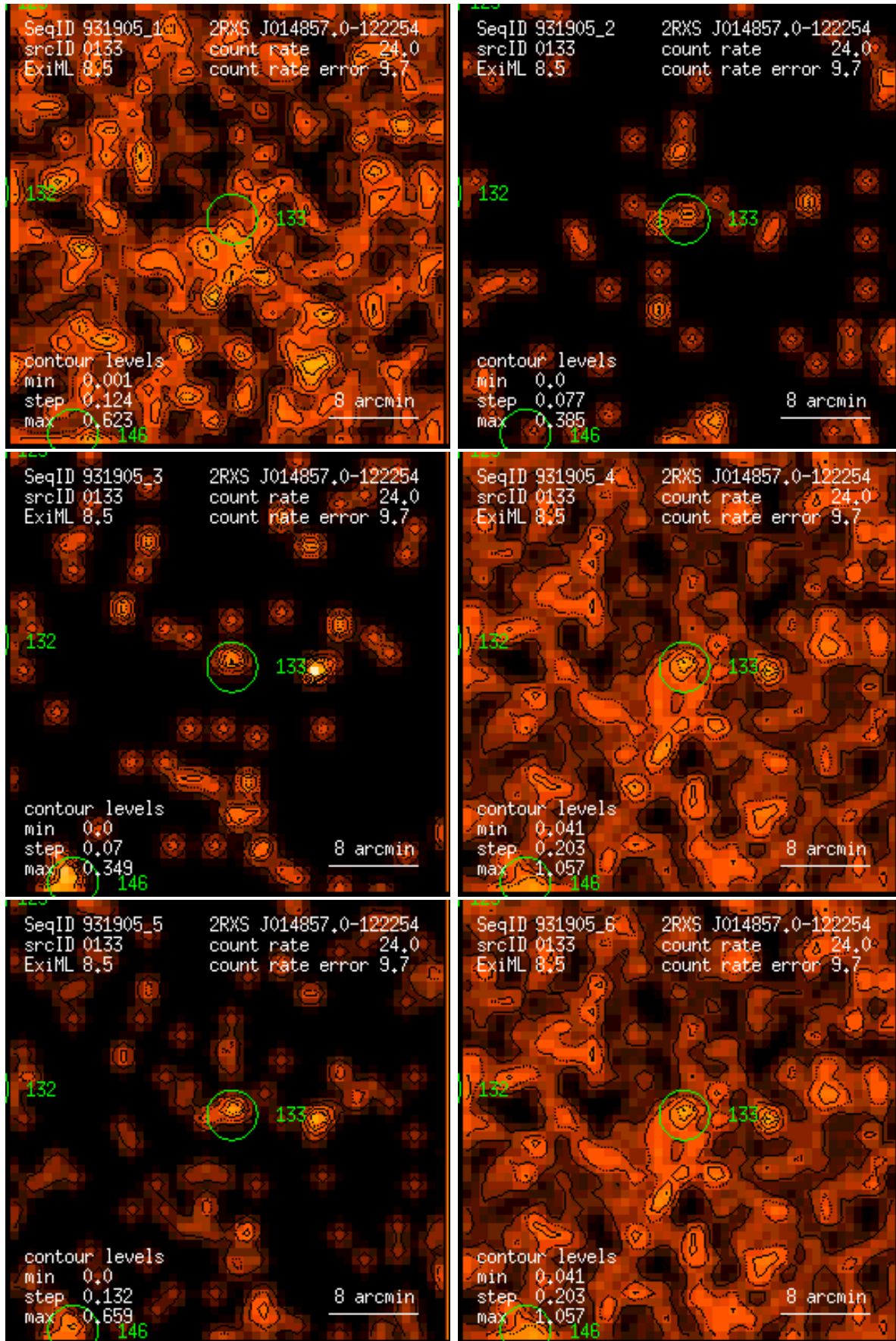
Figure 133: RASS 931905: detection 0133: band rate images, Gaussian filter: (1) PSPC channels 11 – 41, (2) 52 – 90, (3) 91 – 201, (4) 11 – 235, (5) 52 – 201, (6) 11 – 201. Broad band rates in counts/ks. Band rate contour levels in counts/ks/arcmin 2 .
