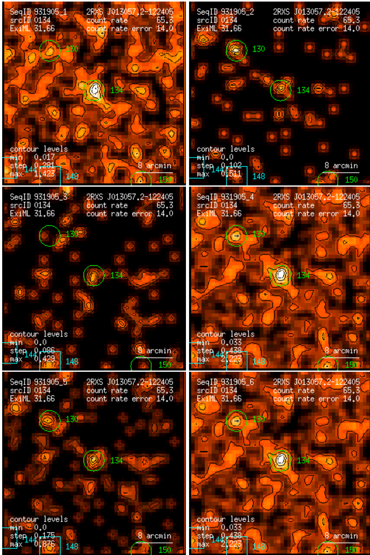
Figure 134: RASS 931905: detection 0134: band rate images, Gaussian filter: (1) PSPC channels 11 – 41, (2) 52 – 90, (3) 91 – 201, (4) 11 – 235, (5) 52 – 201, (6) 11 – 201. Broad band rates in counts/ks. Band rate contour levels in counts/ks/arcmin 2 .
