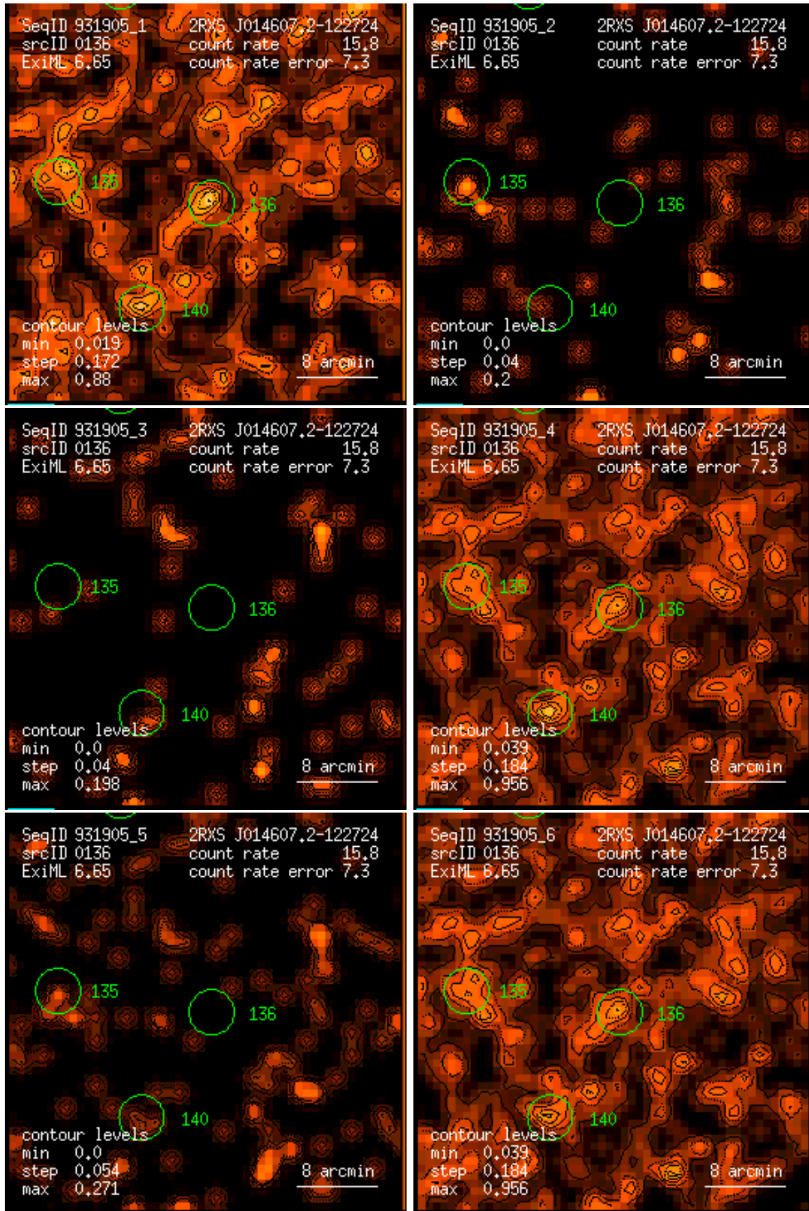
Figure 136: RASS 931905: detection 0136: band rate images, Gaussian filter: (1) PSPC channels 11 – 41, (2) 52 – 90, (3) 91 – 201, (4) 11 – 235, (5) 52 – 201, (6) 11 – 201. Broad band rates in counts/ks. Band rate contour levels in counts/ks/arcmin 2 .
