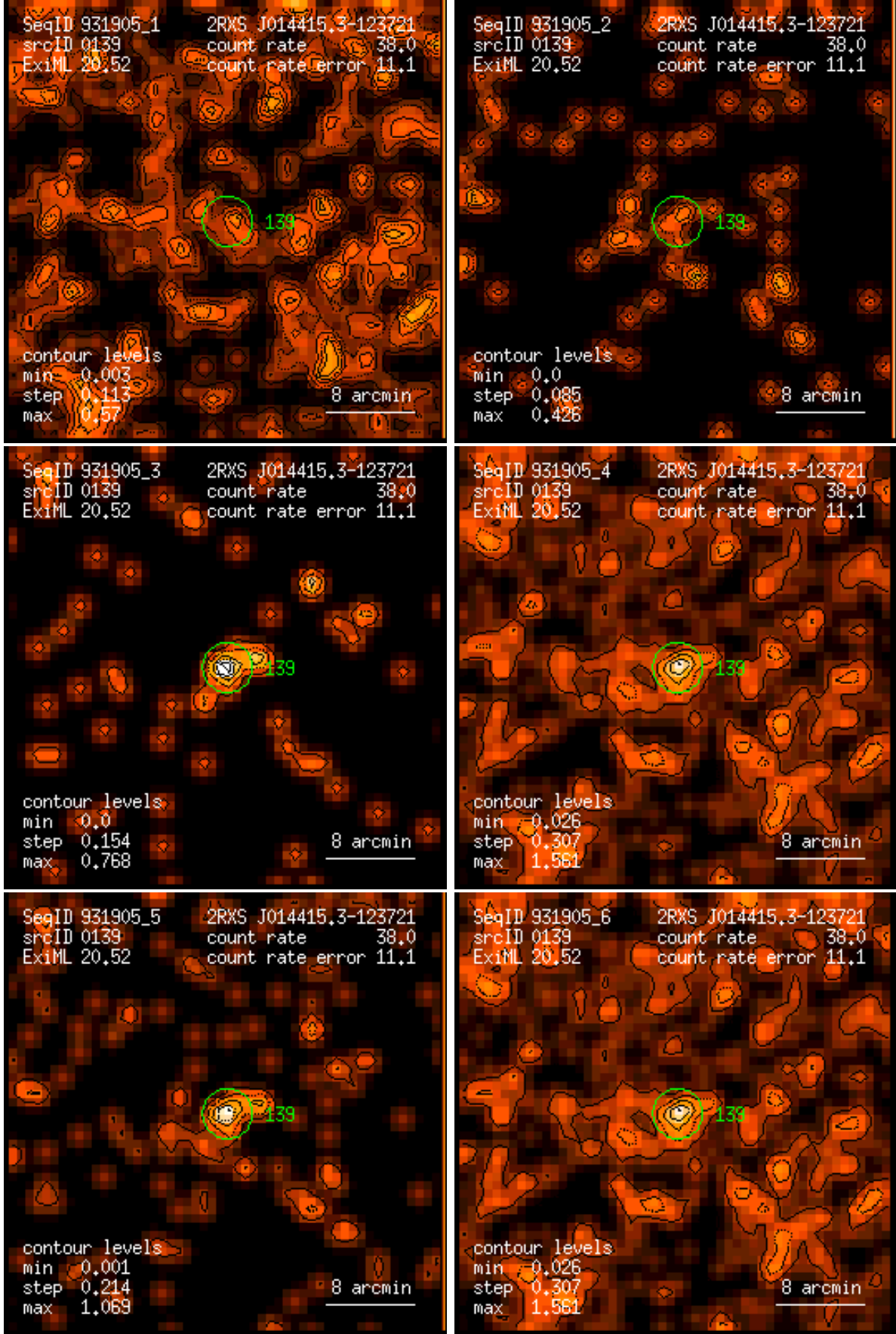
Figure 139: RASS 931905: detection 0139: band rate images, Gaussian filter: (1) PSPC channels 11 – 41, (2) 52 – 90, (3) 91 – 201, (4) 11 – 235, (5) 52 – 201, (6) 11 – 201. Broad band rates in counts/ks. Band rate contour levels in counts/ks/arcmin 2 .
