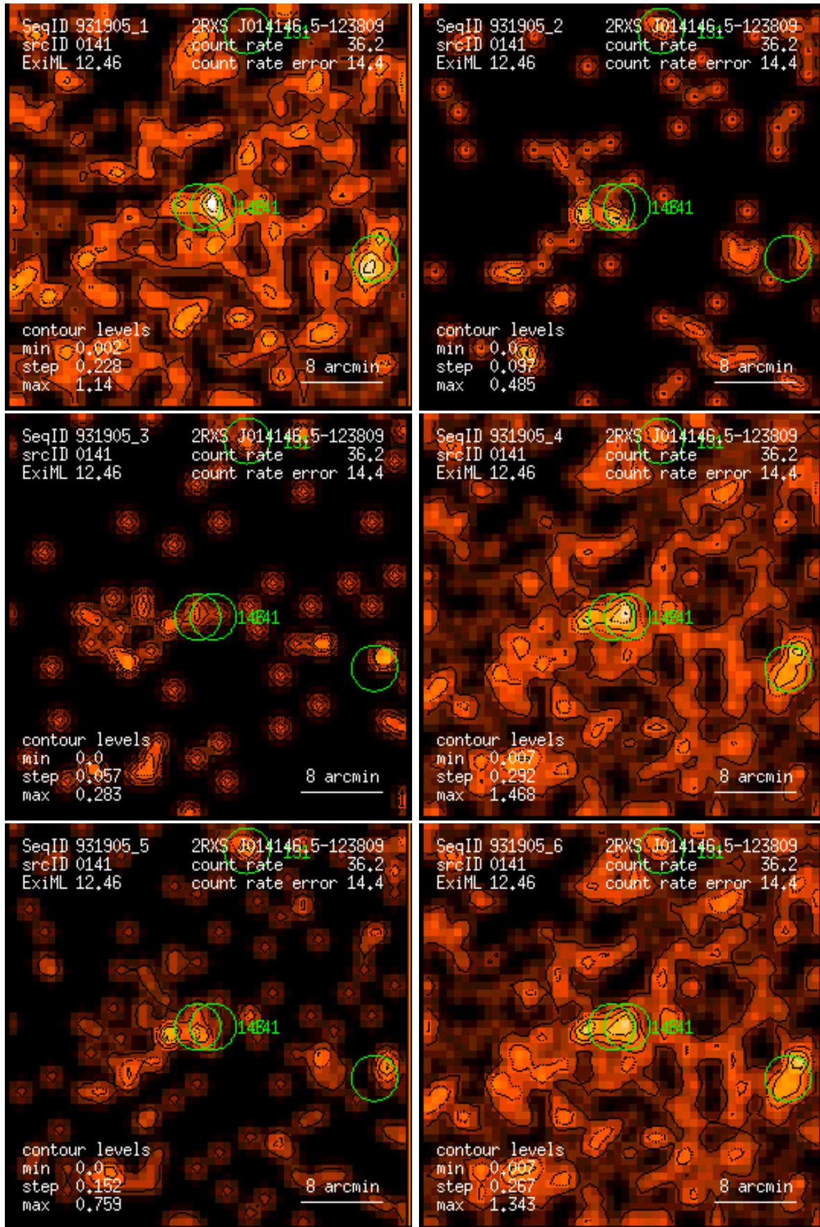
Figure 141: RASS 931905: detection 0141: band rate images, Gaussian filter: (1) PSPC channels 11 – 41, (2) 52 – 90, (3) 91 – 201, (4) 11 – 235, (5) 52 – 201, (6) 11 – 201. Broad band rates in counts/ks. Band rate contour levels in counts/ks/arcmin 2 .
