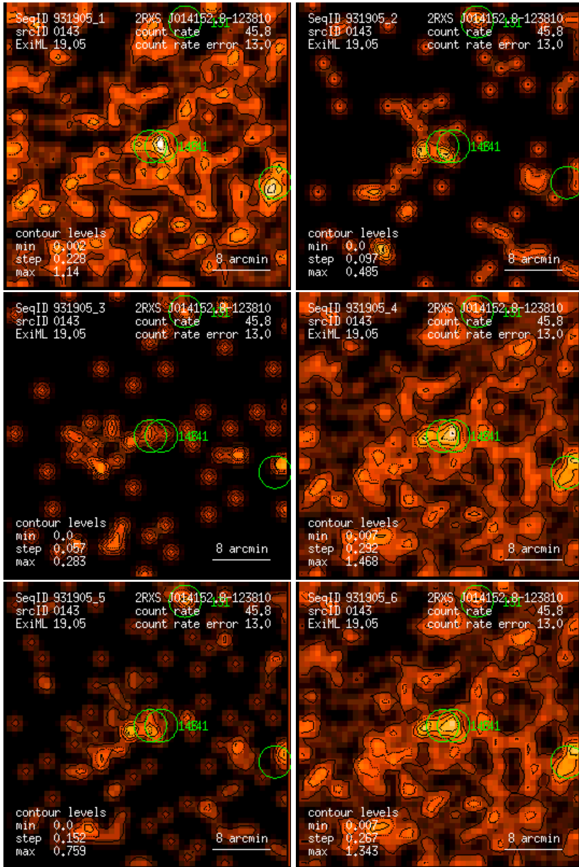
Figure 143: RASS 931905: detection 0143: band rate images, Gaussian filter: (1) PSPC channels 11 – 41, (2) 52 – 90, (3) 91 – 201, (4) 11 – 235, (5) 52 – 201, (6) 11 – 201. Broad band rates in counts/ks. Band rate contour levels in counts/ks/arcmin 2 .
