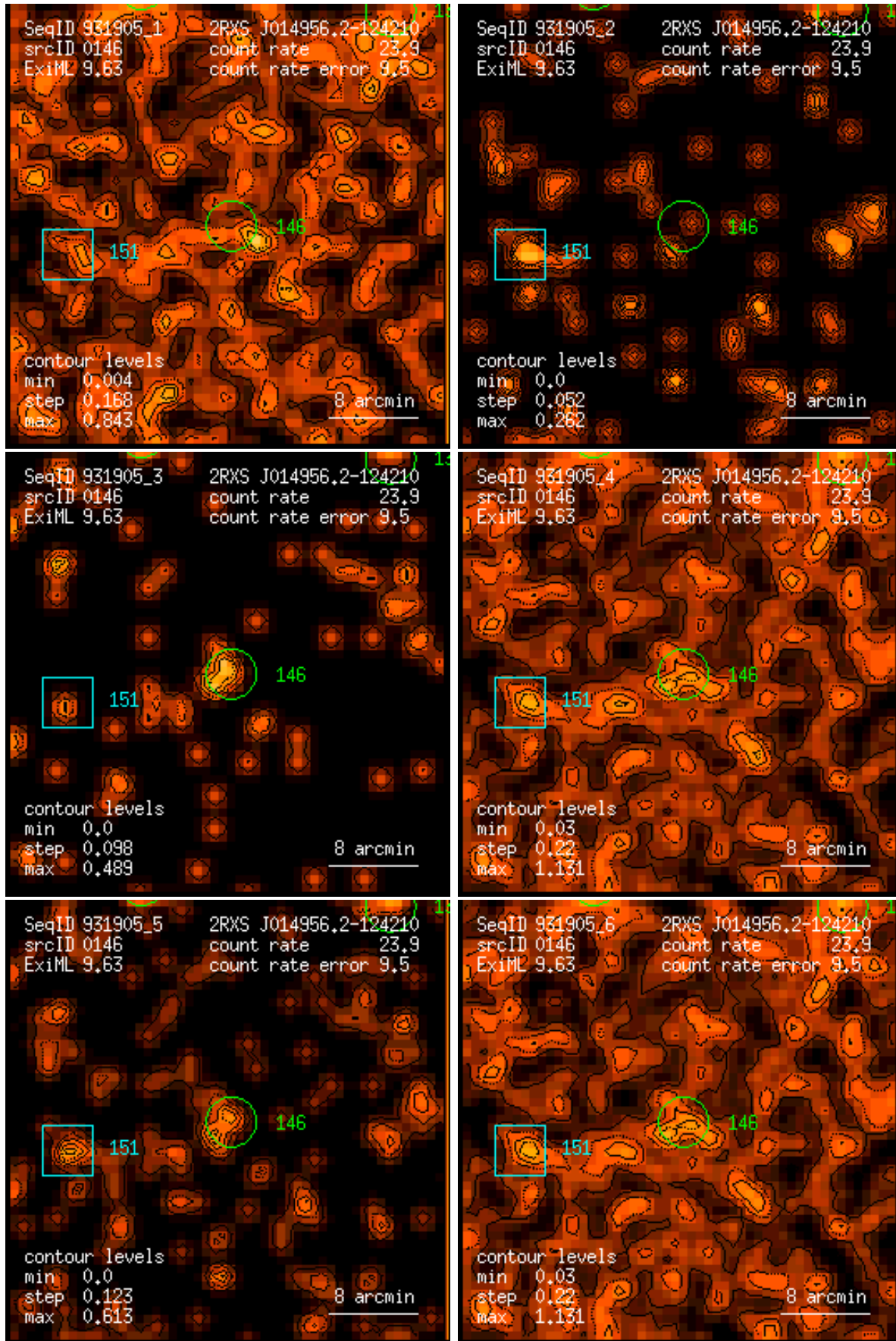
Figure 146: RASS 931905: detection 0146: band rate images, Gaussian filter: (1) PSPC channels 11 – 41, (2) 52 – 90, (3) 91 – 201, (4) 11 – 235, (5) 52 – 201, (6) 11 – 201. Broad band rates in counts/ks. Band rate contour levels in counts/ks/arcmin 2 .
