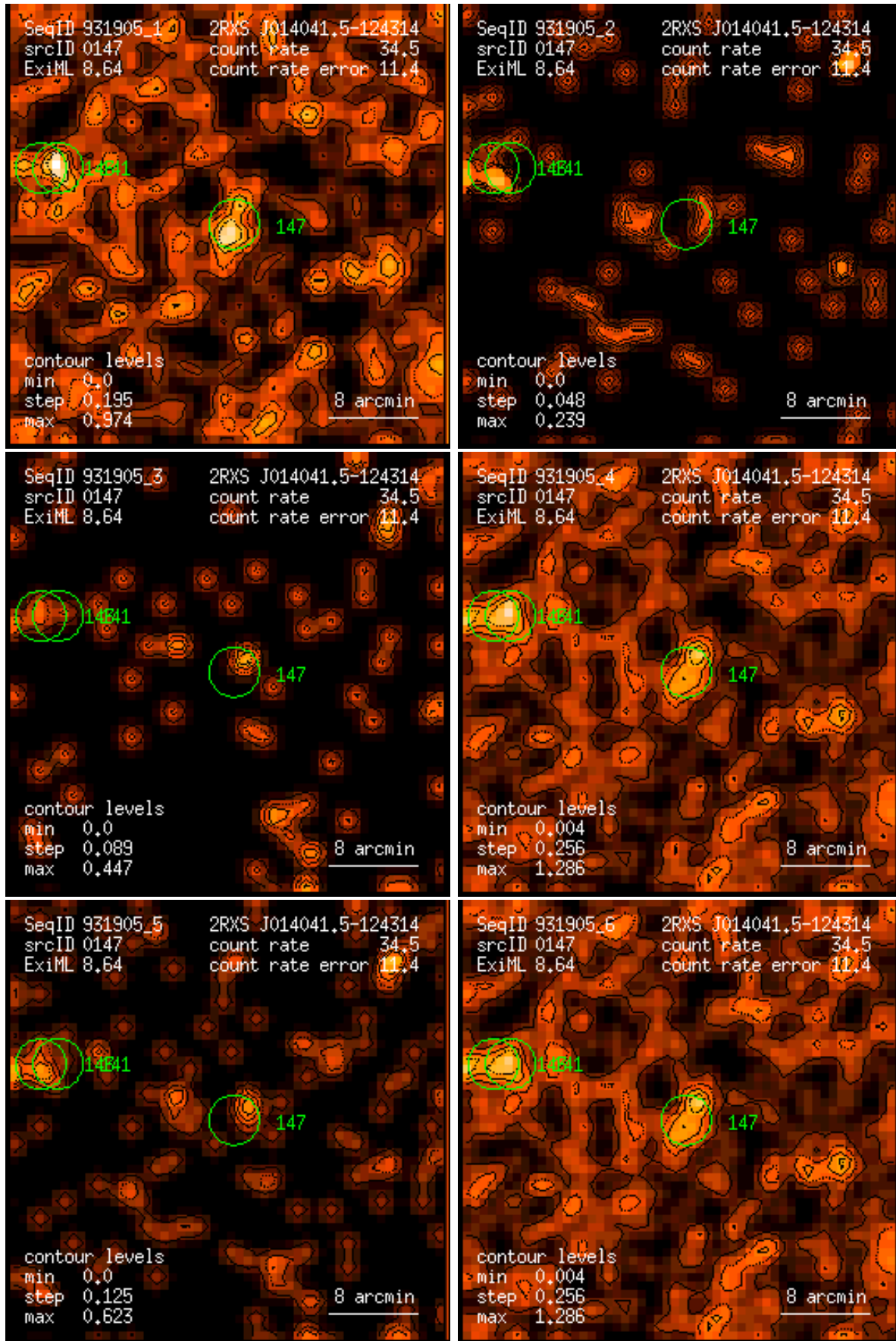
Figure 147: RASS 931905: detection 0147: band rate images, Gaussian filter: (1) PSPC channels 11 – 41, (2) 52 – 90, (3) 91 – 201, (4) 11 – 235, (5) 52 – 201, (6) 11 – 201. Broad band rates in counts/ks. Band rate contour levels in counts/ks/arcmin 2 .
