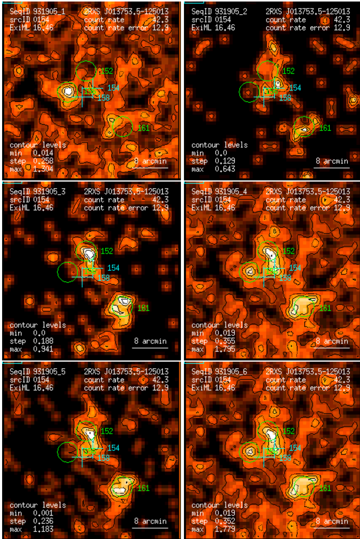
Figure 154: RASS 931905: detection 0154: band rate images, Gaussian filter: (1) PSPC channels 11 – 41, (2) 52 – 90, (3) 91 – 201, (4) 11 – 235, (5) 52 – 201, (6) 11 – 201. Broad band rates in counts/ks. Band rate contour levels in counts/ks/arcmin 2 .
