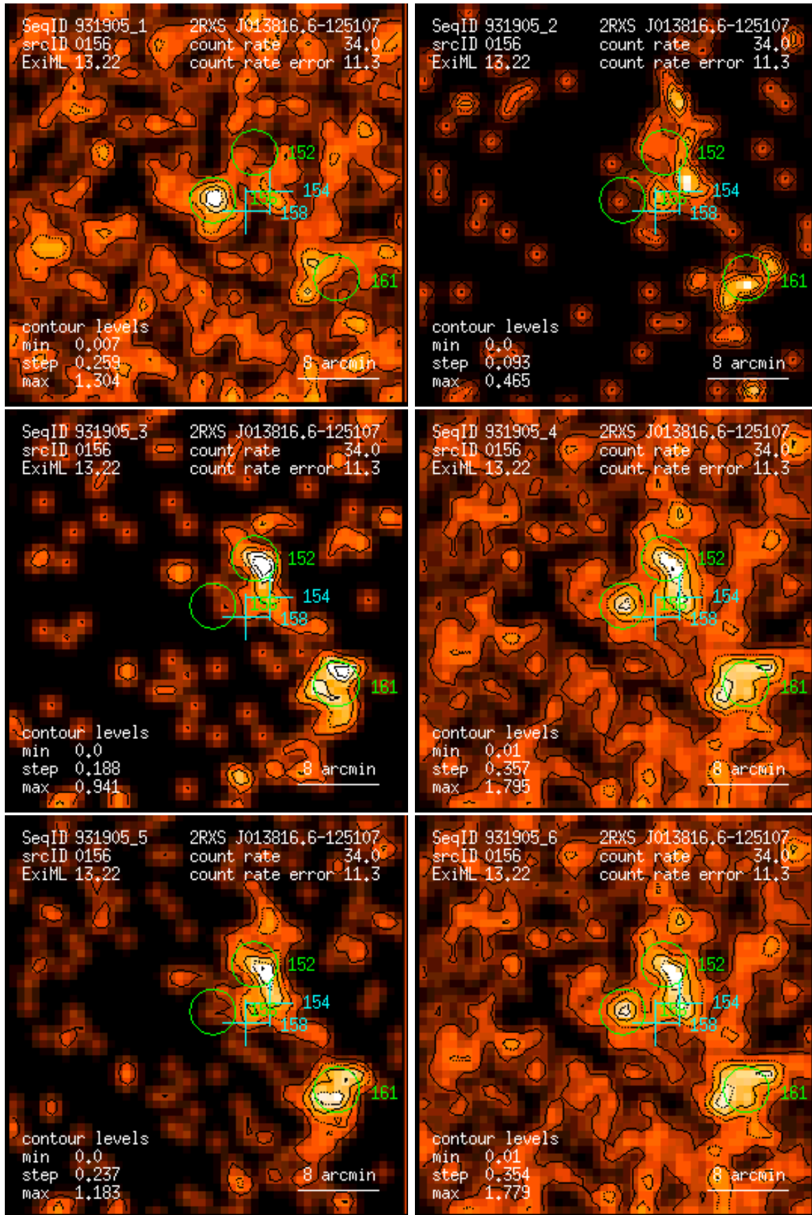
Figure 156: RASS 931905: detection 0156: band rate images, Gaussian filter: (1) PSPC channels 11 – 41, (2) 52 – 90, (3) 91 – 201, (4) 11 – 235, (5) 52 – 201, (6) 11 – 201. Broad band rates in counts/ks. Band rate contour levels in counts/ks/arcmin 2 .
